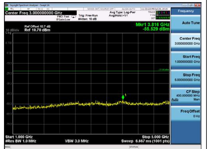
CUE-802.11n-20-5580M-chain1(1GHz-5GHz)
