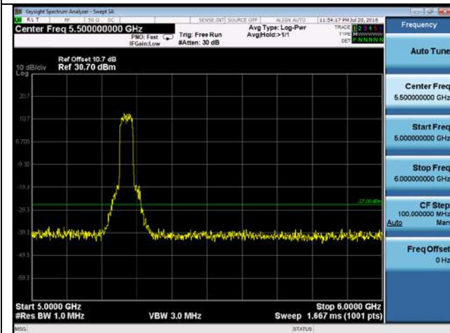
CUE-802.11n-40-5270M-chain1(5GHz-6GHz)
