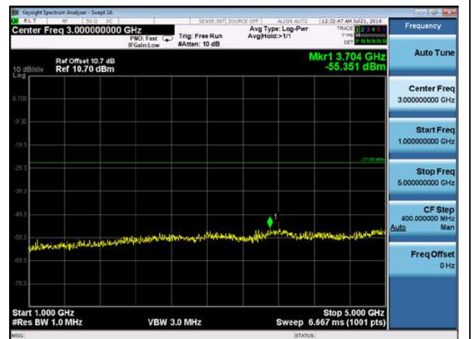
CUE-802.11n-40-5270M-chain2(1GHz-5GHz)
