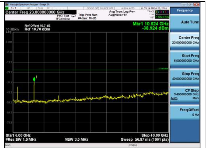
CUE-802.11n-40-5310M -chain1(6GHz-40GHz)
