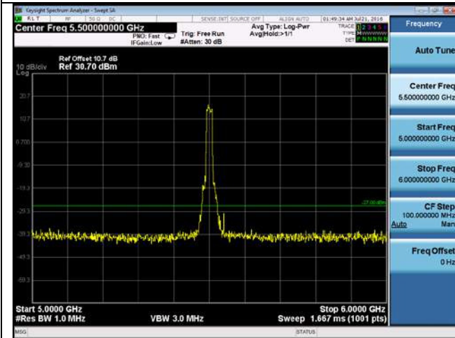
CUE-802.11n-20-5500M-chain4(5GHz-6GHz)
