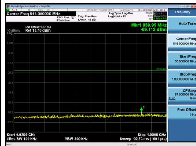
CUE-802.11n-20-5320M-chain 3(30MHz-1GHz)
