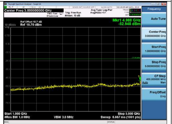
CUE-802.11ac-80-5290M-chain 4(1GHz-5GHz)
