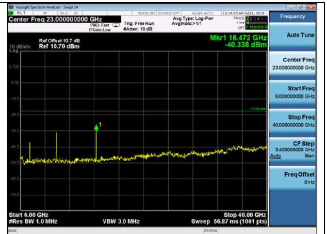
CUE-802.11a-5500M -chain2(6GHz-40GHz)
