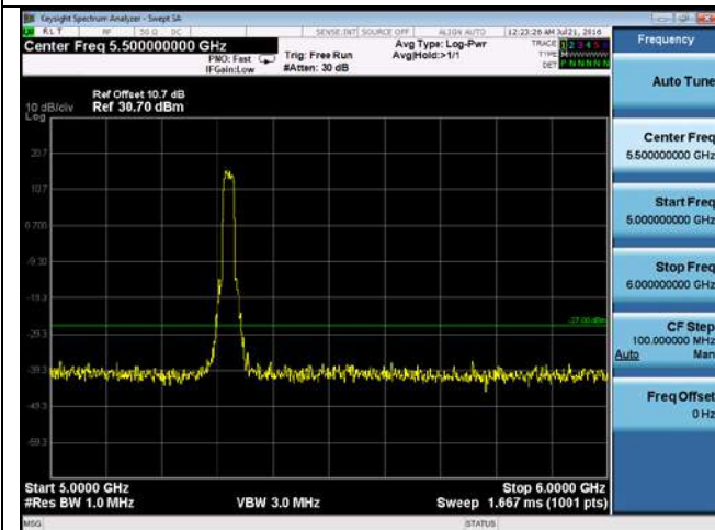
CUE-802.11n-20-5320M-chain 2(5GHz-6GHz)
