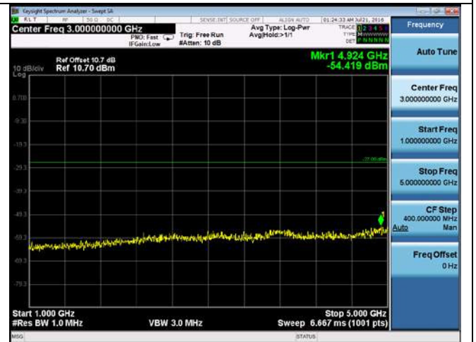
CUE-802.11n-40-5270M-chain3(1GHz-5GHz)
