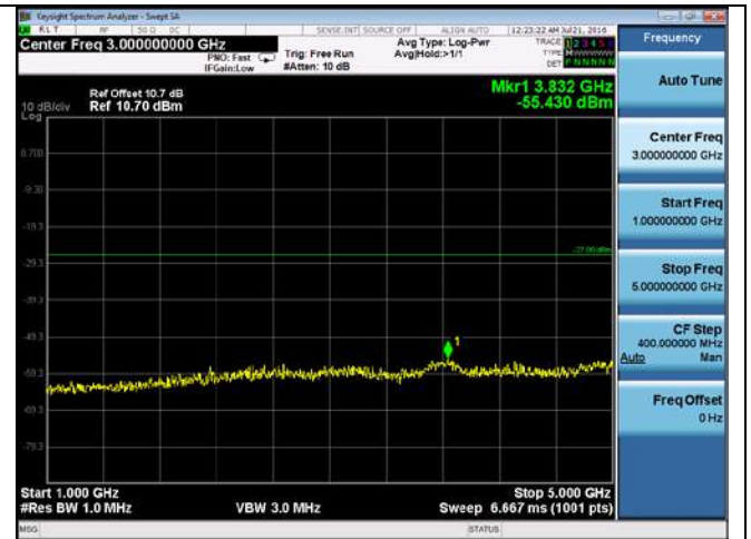
CUE-802.11n-20-5320M-chain 2(1GHz-5GHz)
