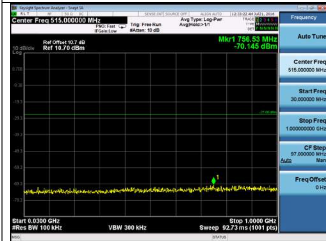
CUE-802.11n-40-5310M -chain2(30MHz-1GHz)
