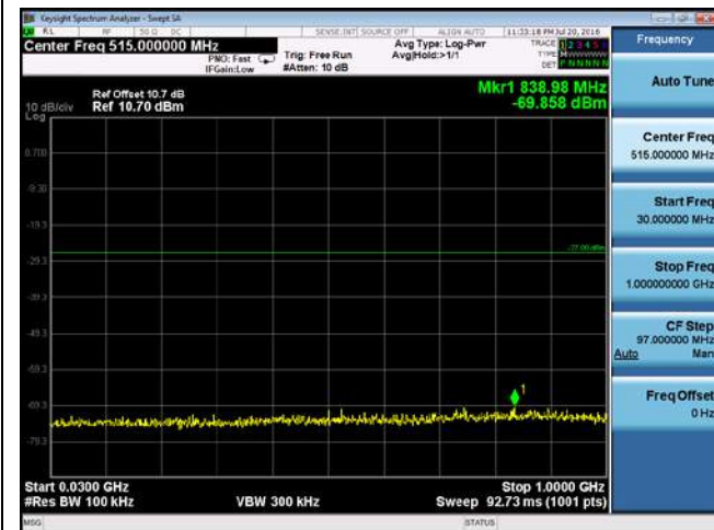
CUE-802.11n-20-5580M-chain1(30MHz-1GHz)
