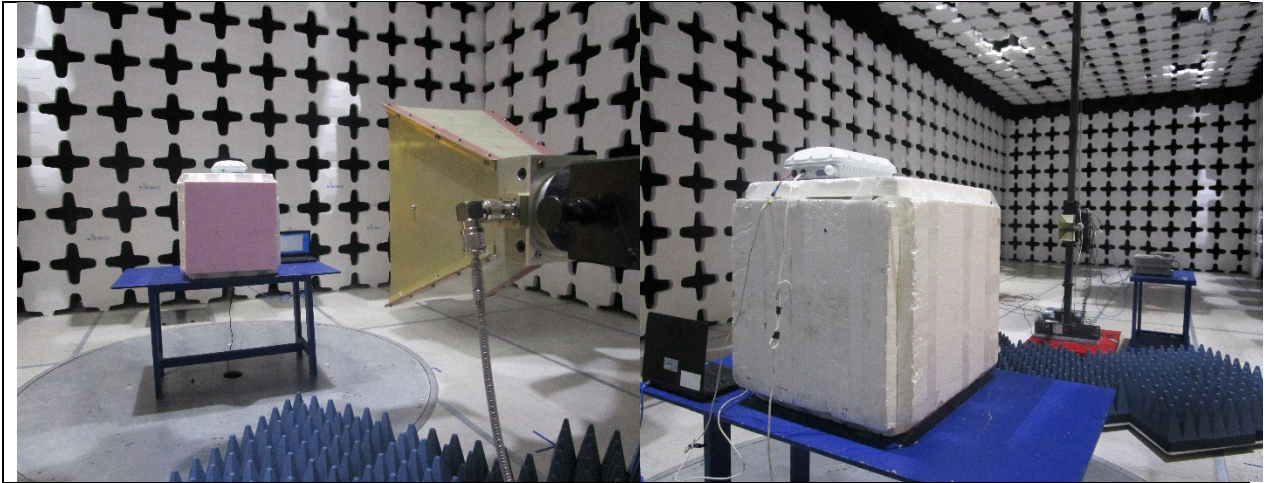
Radiated Emissions (>1GHz) - Front View
