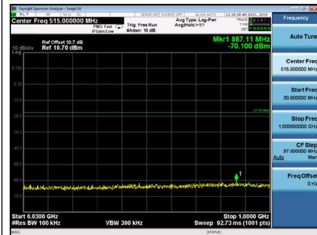
CUE-802.11a-5745M-chain2(30MHz-1GHz)
