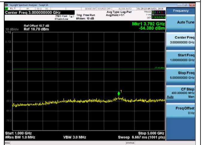
CUE-802.11n-40-5755M -chain3(1GHz-5GHz)
