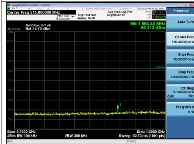
CUE-802.11n-20-5825M -chain 4(30MHz-1GHz)
