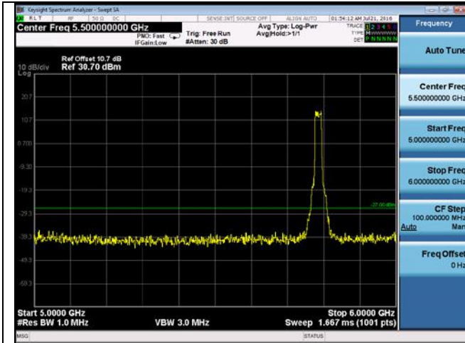
CUE-802.11a-5785M-chain 4(5GHz-6GHz)
