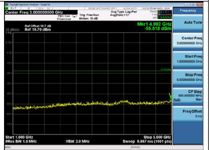
CUE-802.11n-40-5230M chain2(1GHz-5GHz)
