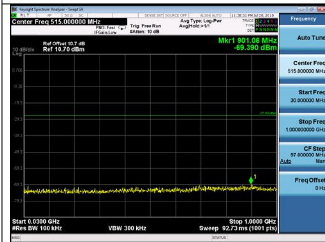
CUE-802.11a-5825M-chain 1(30MHz-1GHz)
