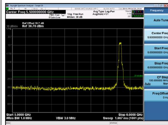
CUE-802.11a-5825M-chain 1(5GHz-6GHz)
