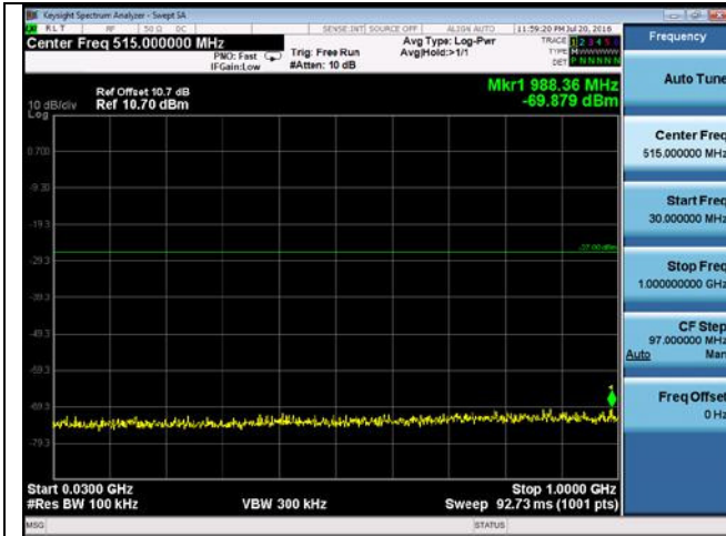
CUE-802.11n-40-5755M-chain1(30MHz-1GHz)
