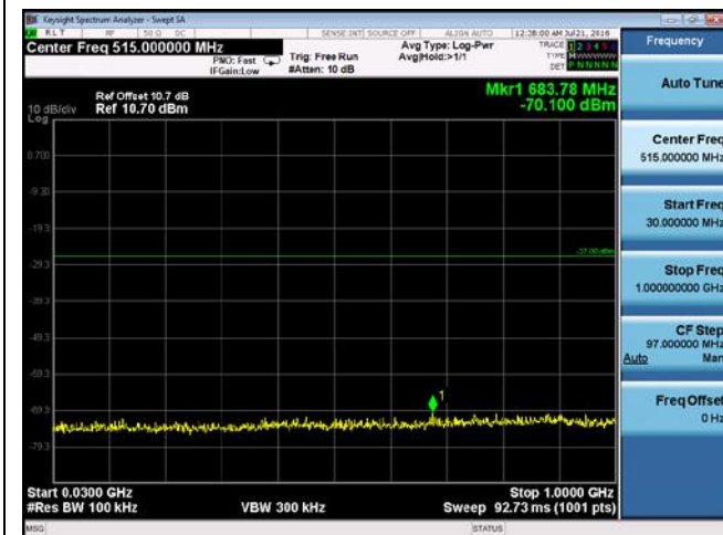
CUE-802.11n-40-5755M-chain2(30MHz-1GHz)
