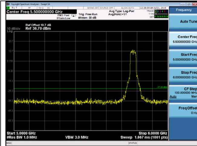
CUE-802.11n-40-5755M -chain2(5GHz-6GHz)
