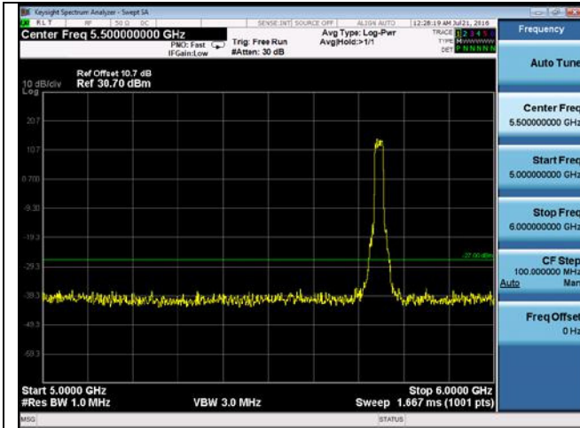
CUE-802.11n-20-5745M -chain2(5GHz-6GHz)
