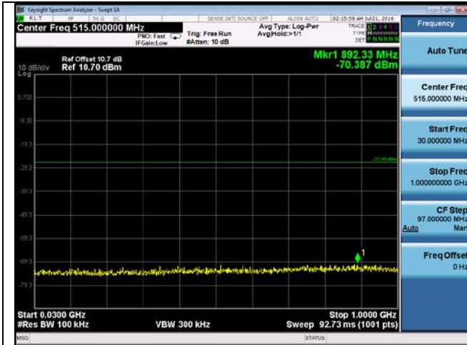
CUE-802.11n-40-5755M -chain4(30MHz-1GHz)
