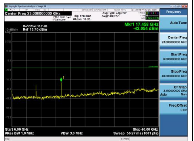
CUE-802.11a-5825M-chain 1(6GHz-40GHz)
