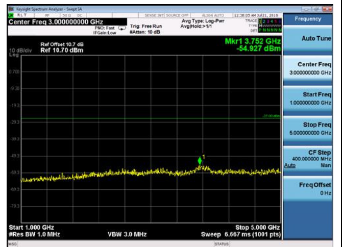
CUE-802.11n-40-5755M-chain2(1GHz-5GHz)
