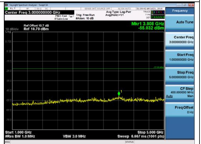
CUE-802.11a-5745M-chain3(1GHz-5GHz)
