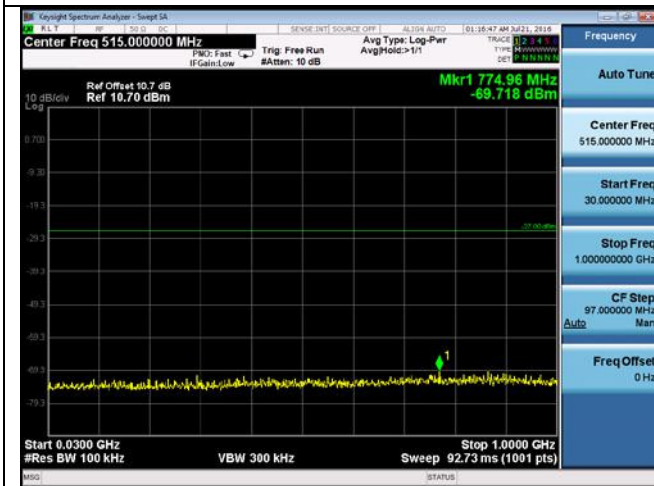
CUE-802.11n-20-5745M -chain3(30MHz-1GHz)
