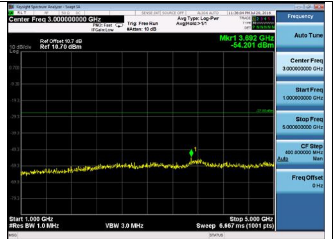
CUE-802.11a-5745M-chain1(1GHz-5GHz)
