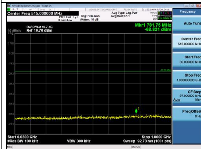
CUE-802.11n-20-5825M -chain 1(30MHz-1GHz)
