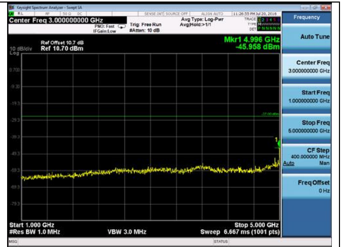
CUE-802.11a-5180M-chain1(1GHz-5GHz)
