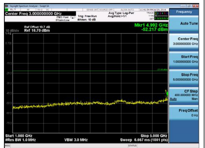
CUE-802.11n-20-5200M-chain1(1GHz-5GHz)
