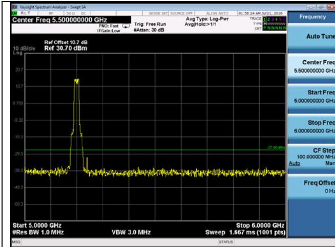
CUE-802.11n-20-5200M-chain 4(5GHz-6GHz)
