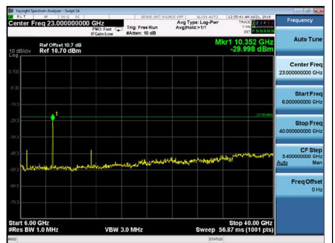
CUE-802.11a-5180M-chain3(6GHz-40GHz)
