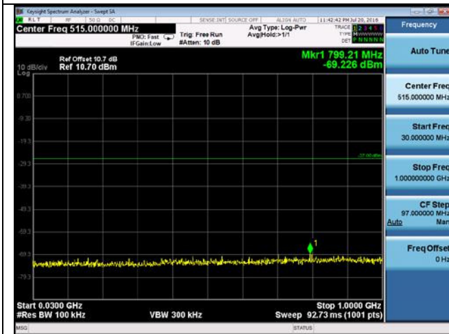
CUE-802.11n-20-5240M-chain 1(30MHz-1GHz)
