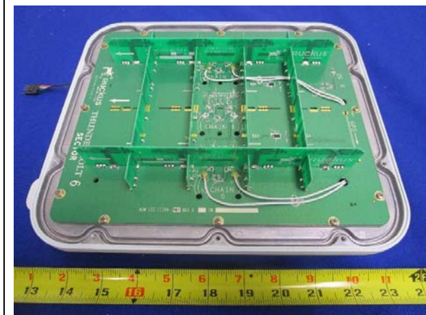
T310S Antenna Set View
