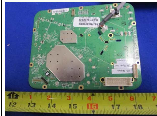
Modem Board Bottom View
