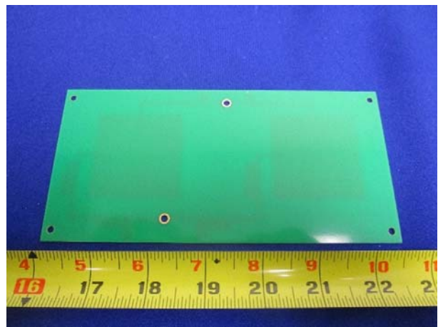
T310N Antenna Part2 Bottom View
