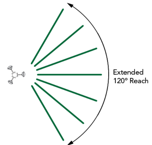
FIGURE 2 Typical AP sector azimuth plane coverage, top view
