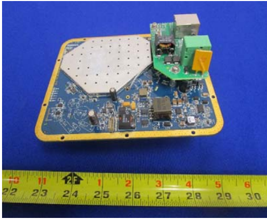
Modem Board Bottom View
