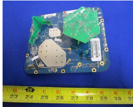
Modem Board Top View
