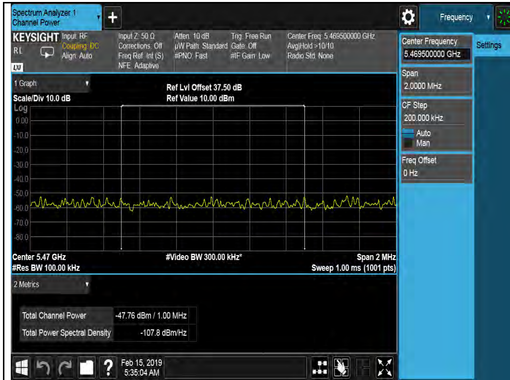
802.11ax-HT20-5500MHz
