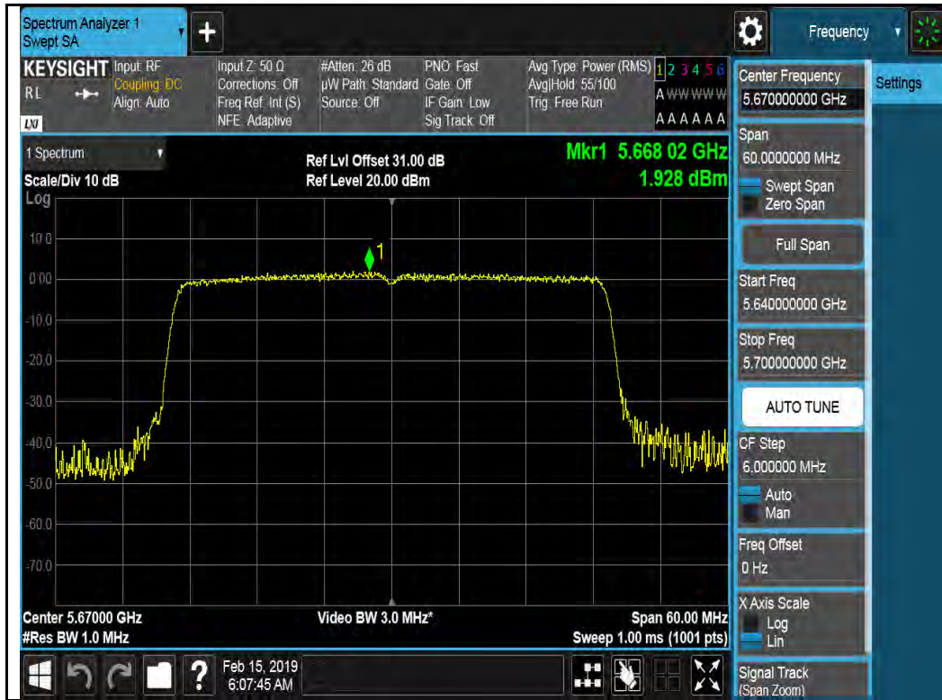
802.11ax-HT40 5670M
