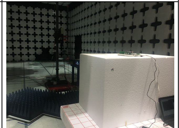
Radiated Emission Above 1G – Rear View
