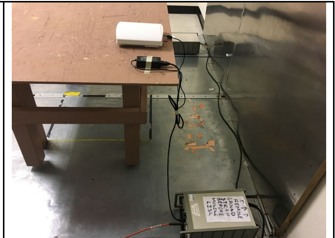
Conducted Emission – Side View
