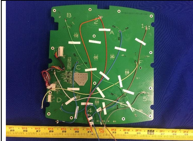
Antenna board- bottom view
