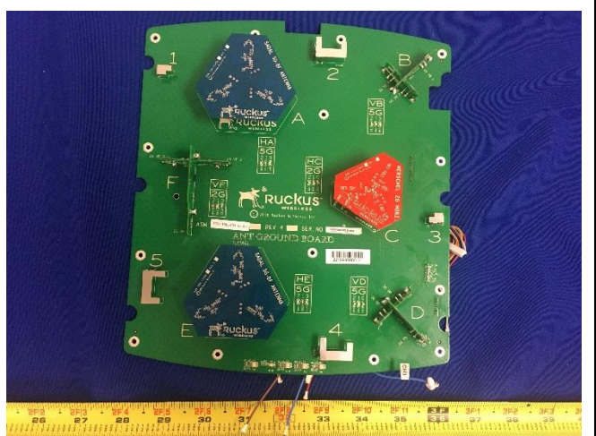
Antenna board- top view
