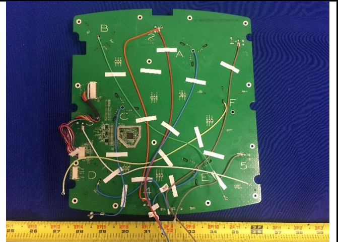
Antenna board cover off - bottom view
