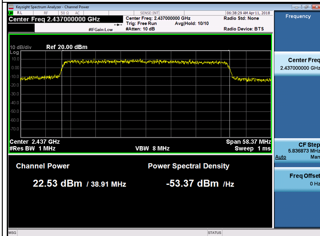
802.11ax40 2437MHz Chain 1
