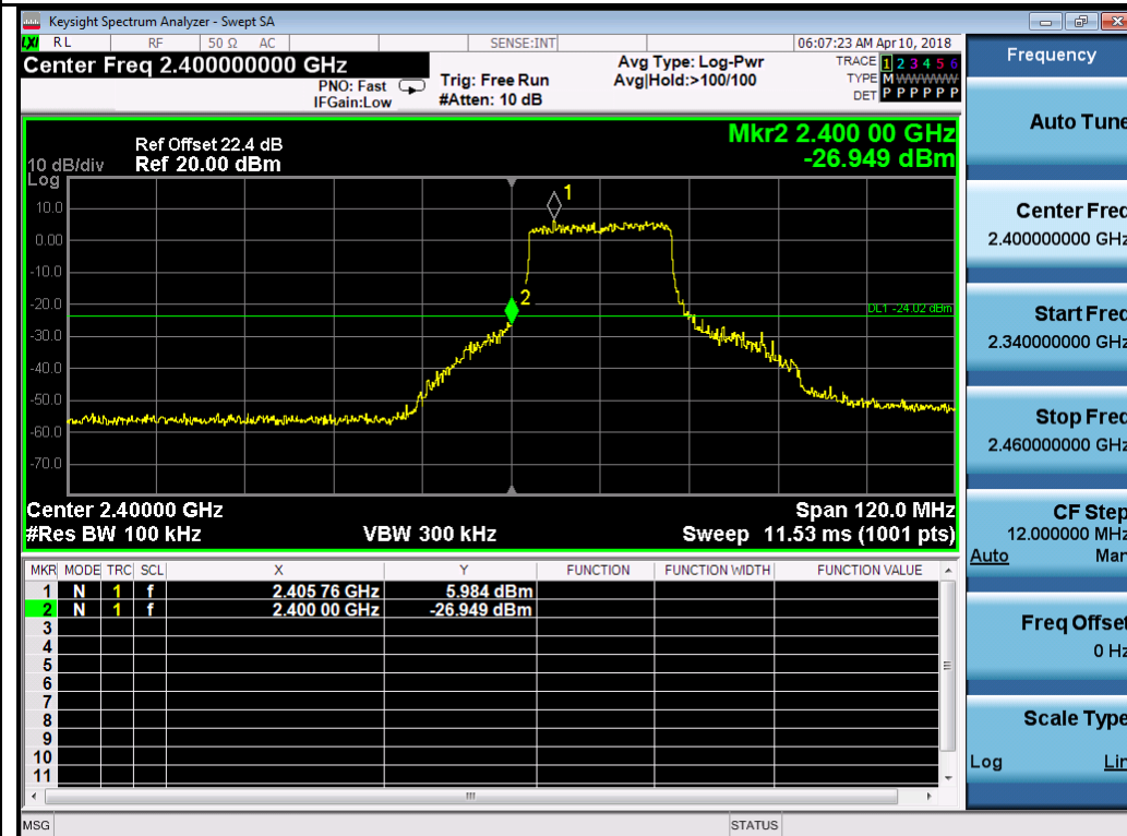
802.11ax20-2412MHz Chain 3
