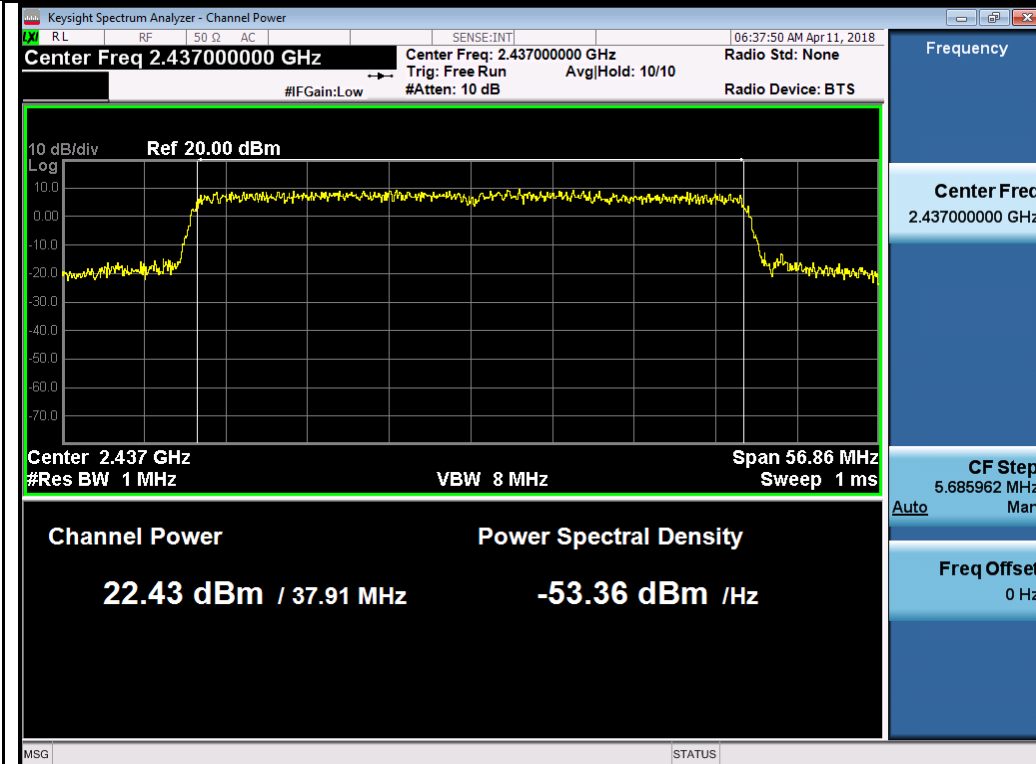
802.11ax40 2437MHz Chain 2
