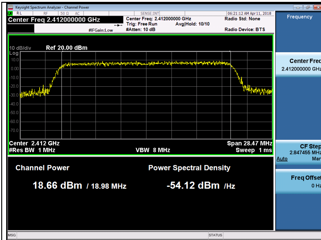
802.11ax20 2412MHz Chain 0
