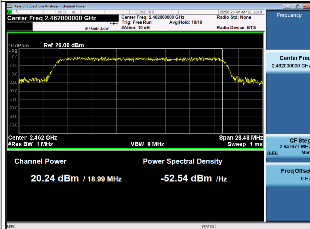
802.11ax20 2462MHz Chain 1
