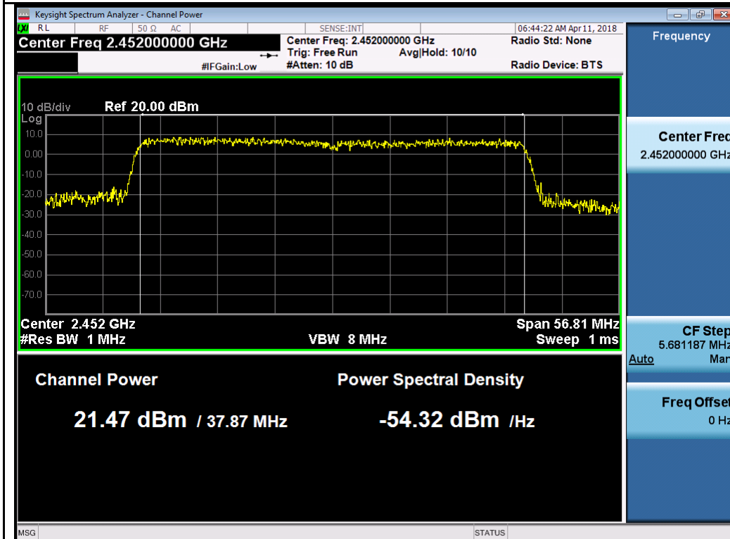
802.11ax40 2452MHz Chain 3
