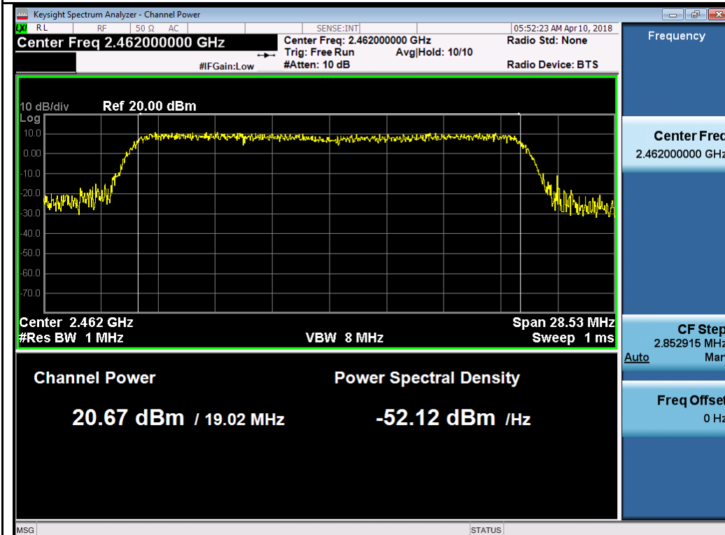
802.11ax20 2462MHz Chain 3
