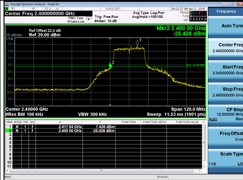
802.11ax20-2412MHz Chain 0
