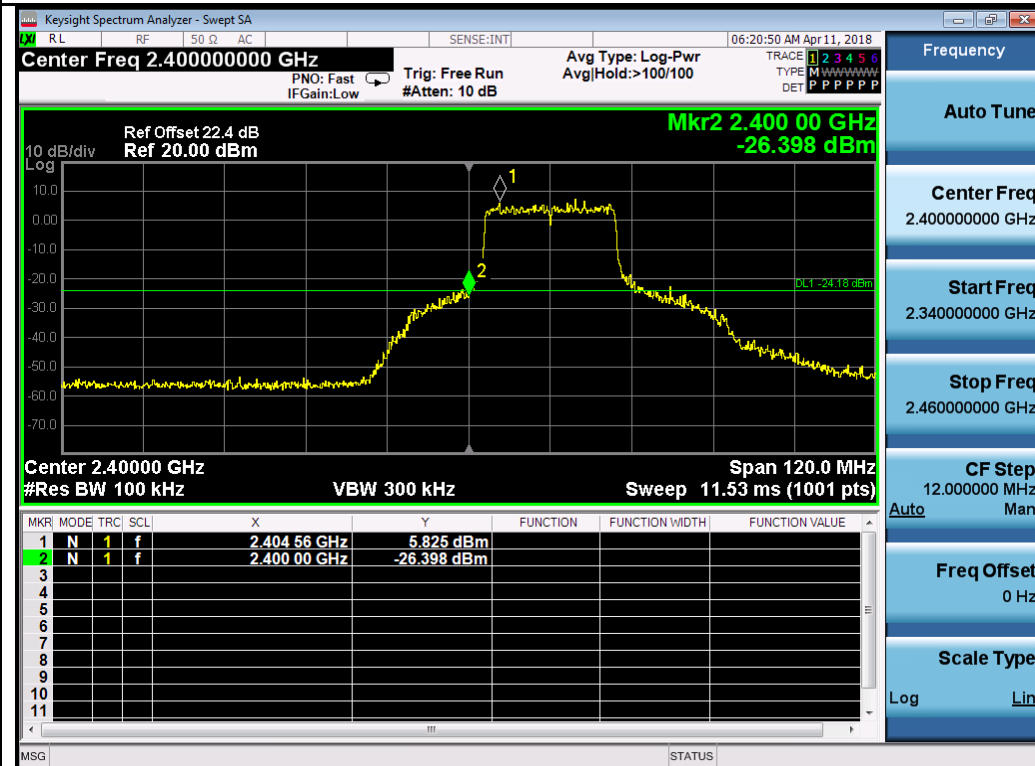
802.11ax20-2412MHz Chain 1
