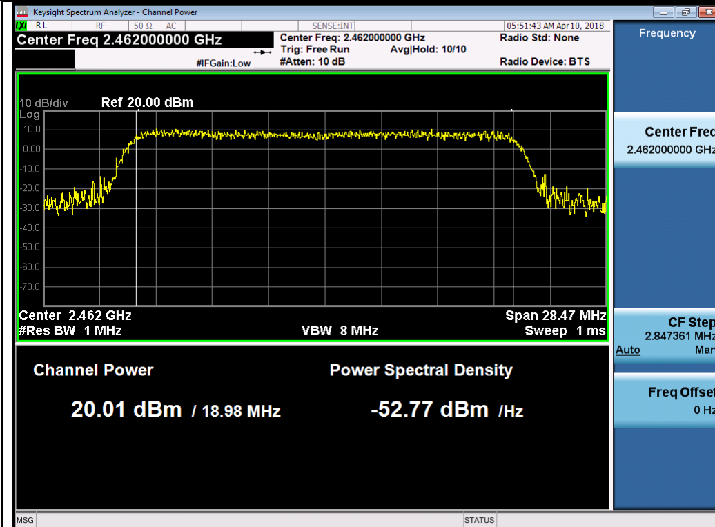
802.11ax20 2462MHz Chain 2
