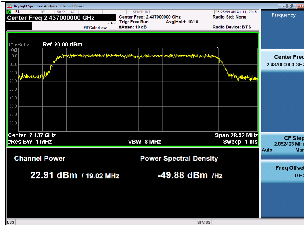
802.11ax20 2437MHz Chain 3
