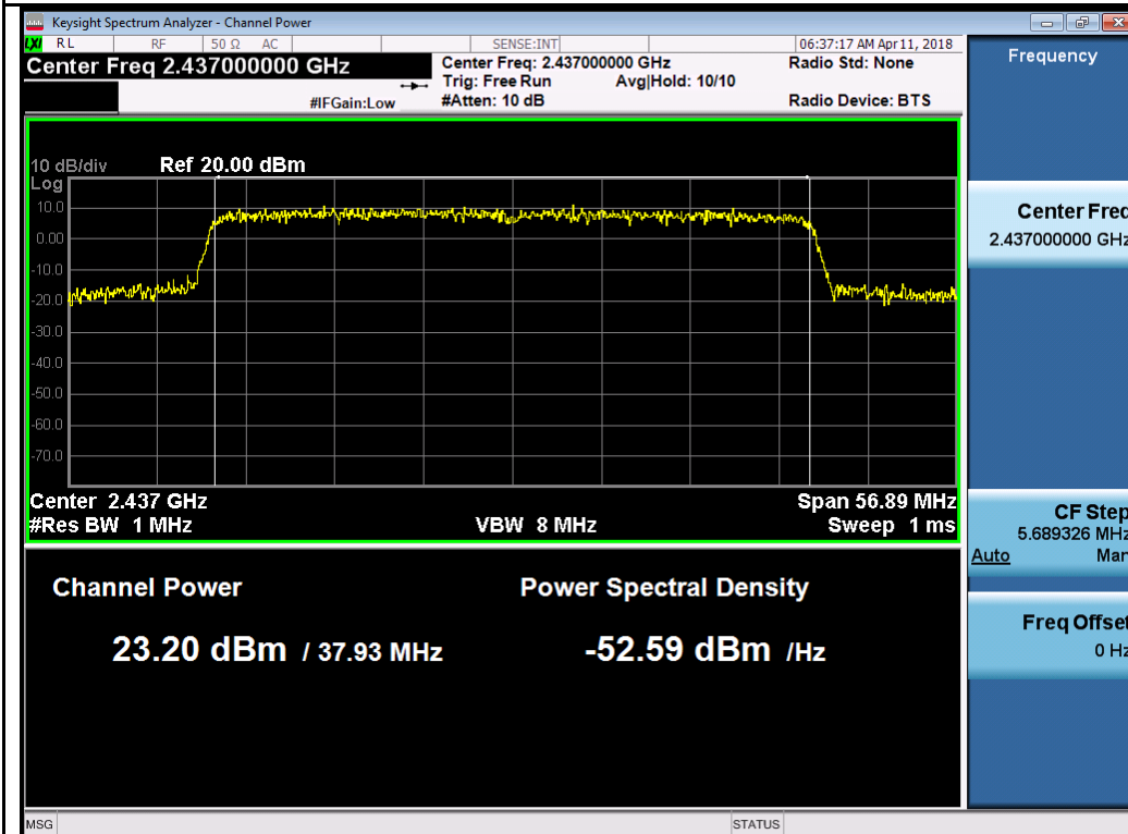
802.11ax40 2437MHz Chain 3
