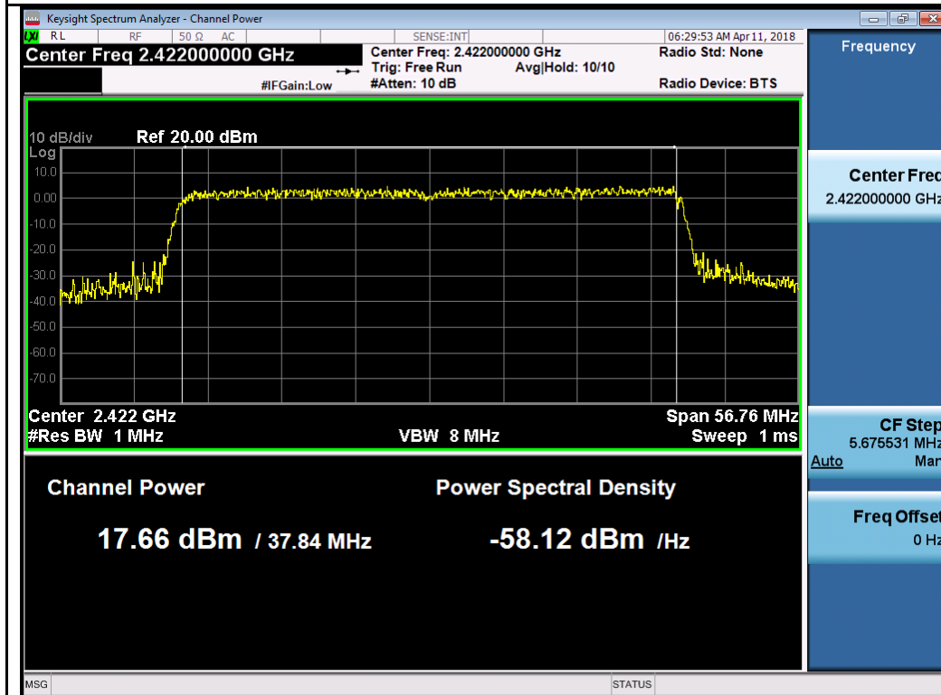
802.11ax40 2422MHz Chain 0
