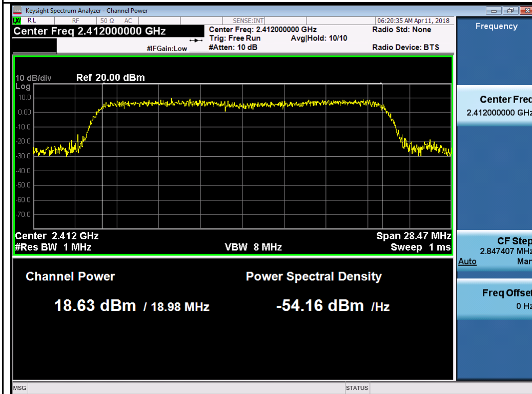
802.11ax20 2412MHz Chain 1
