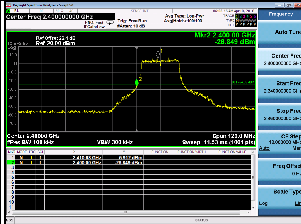
802.11ax20-2412MHz Chain 2
