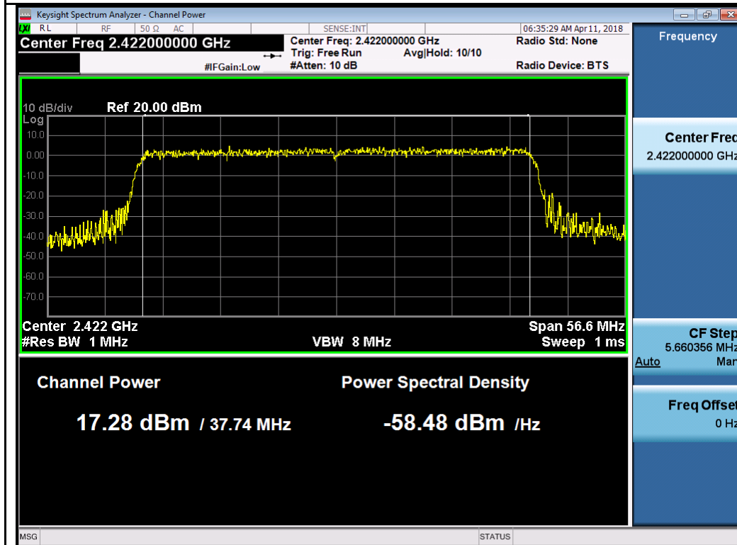
802.11ax40 2422MHz Chain 2
