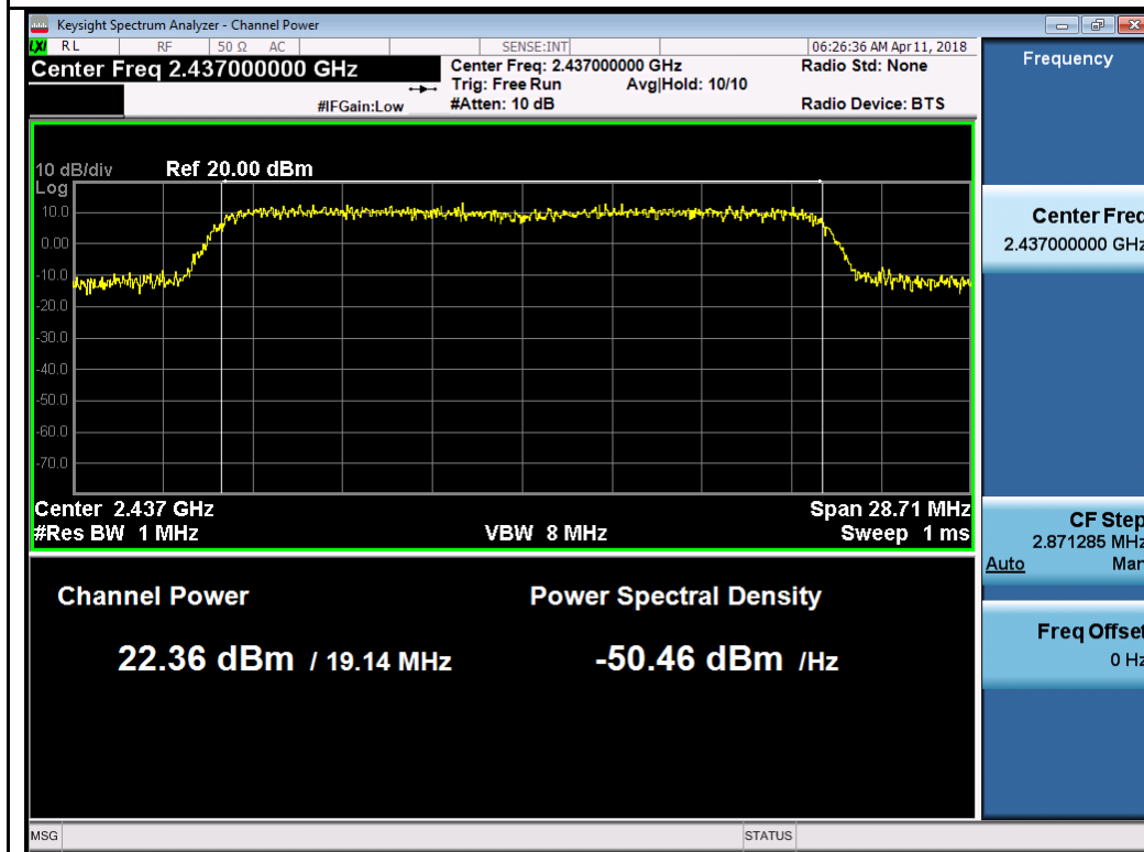
802.11ax20 2437MHz Chain 1
