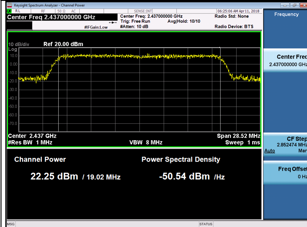
802.11ax20 2437MHz Chain 2
