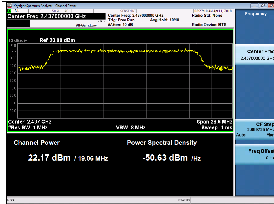
802.11ax20 2437MHz Chain 0
