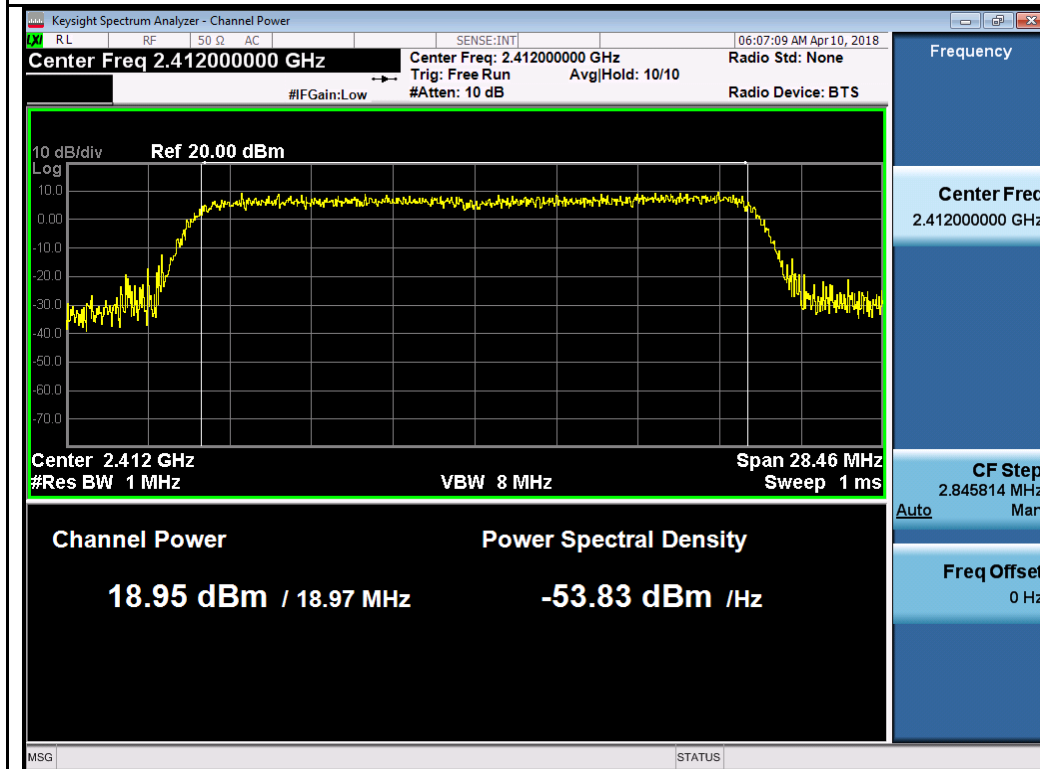
802.11ax20 2412MHz Chain 3
