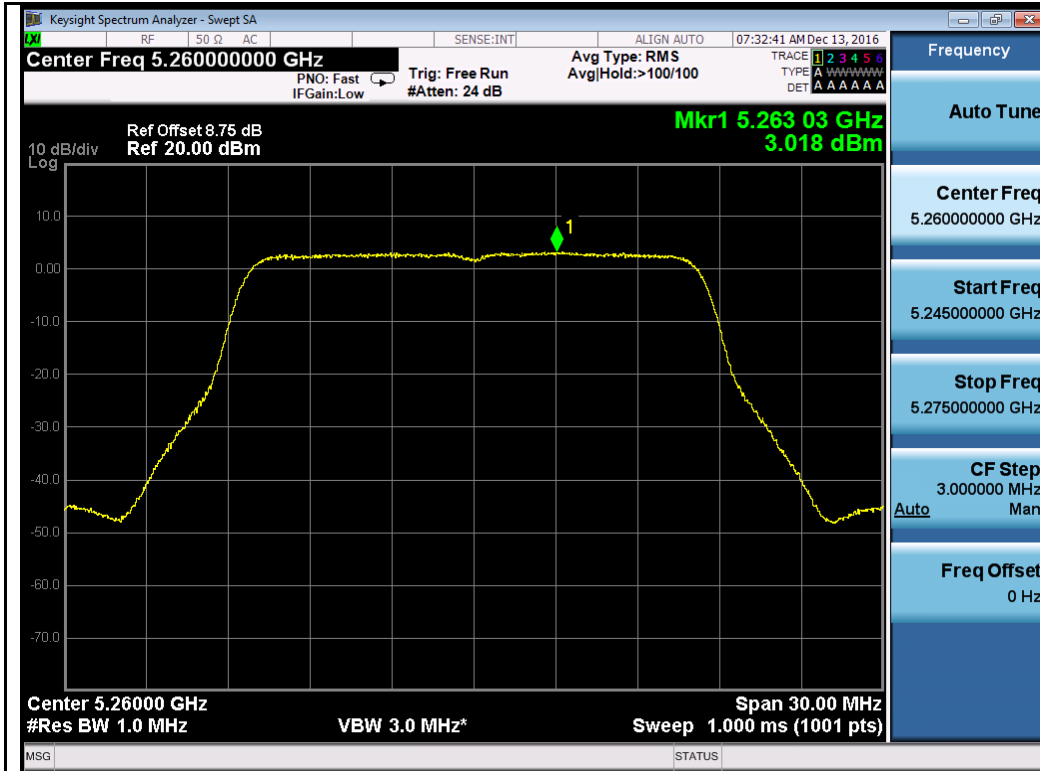
802.11a-5260M
