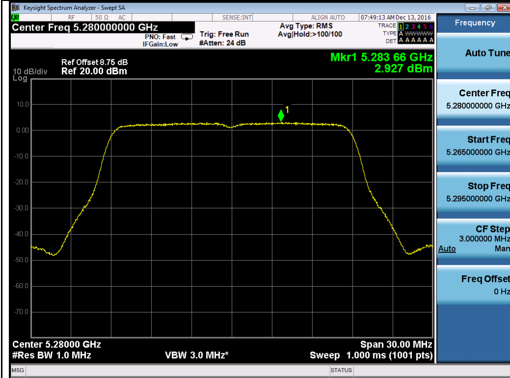
802.11n-HT20 5280M
