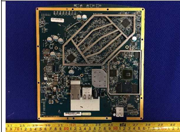
EUT Main Board - Shielding off Bottom View
