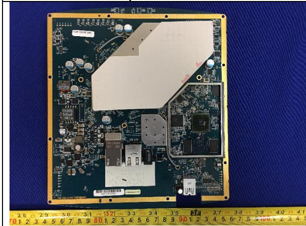
EUT Main Board - Bottom View
