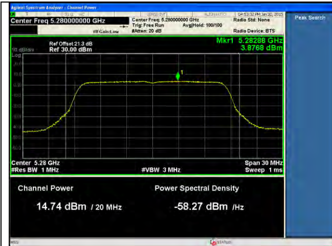
PSD-802.11a-5280M-chain3
