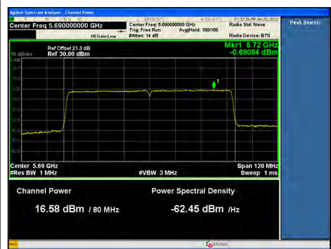
PSD-802.11ac-CROSSOVER-5690M-chain4
