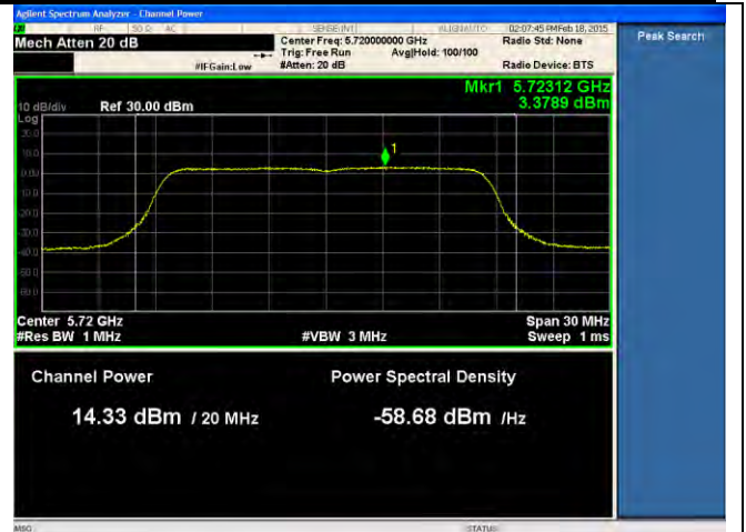
PSD-802.11a-CROSSOVER-5720M-chain4
