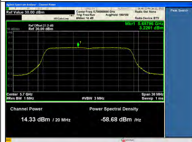
PSD-802.11a-5700M-chain1
