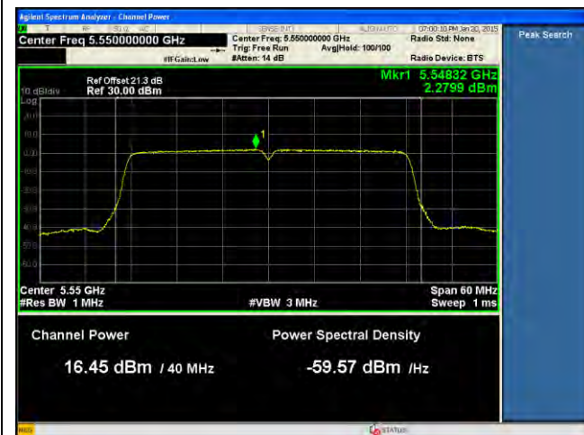
PSD-802.11n-40M-5550M-chain1
