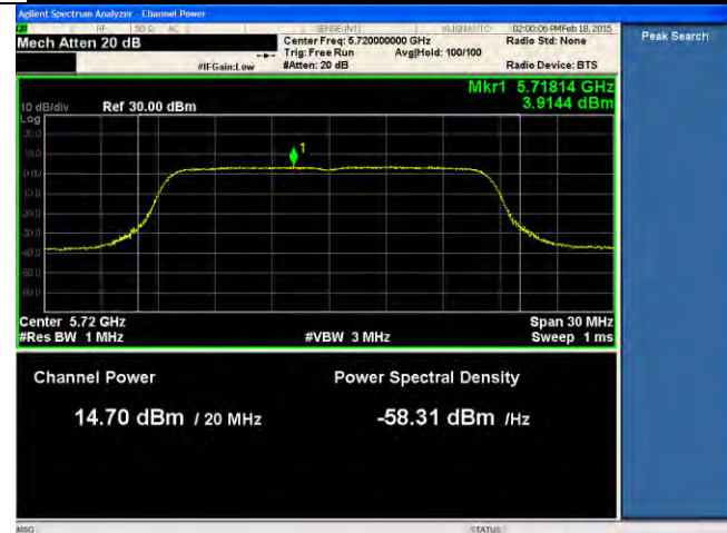
PSD-802.11a-CROSSOVER-5720M-chain3
