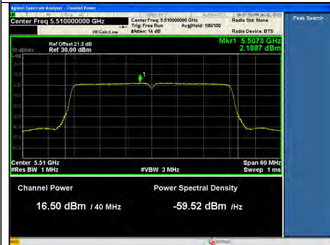
PSD-802.11n-40M-5510M-chain3
