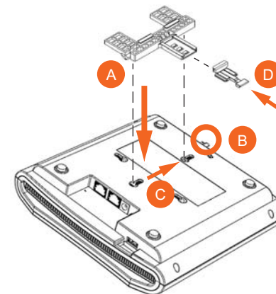
Figure 3. Attaching the T-bar bracket to the AP
