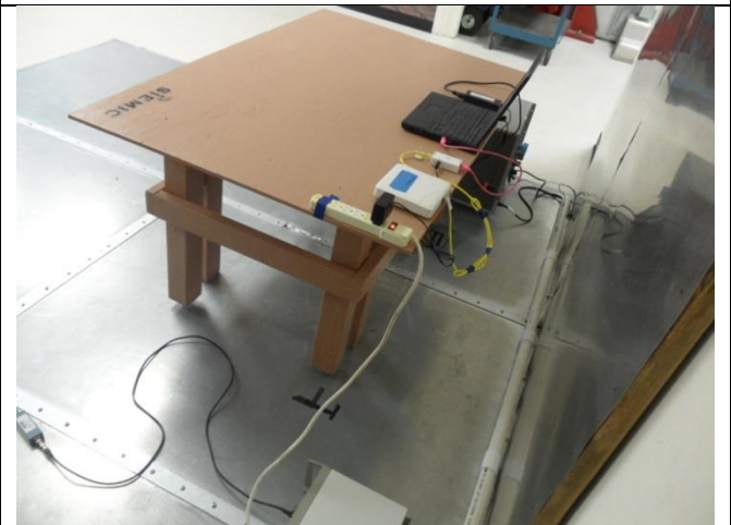
Conducted Emission – Rear View with PoE Adapter
