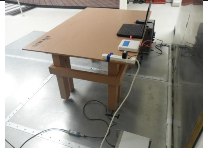
Conducted Emission – Bottom View with AC/DC Adapter
