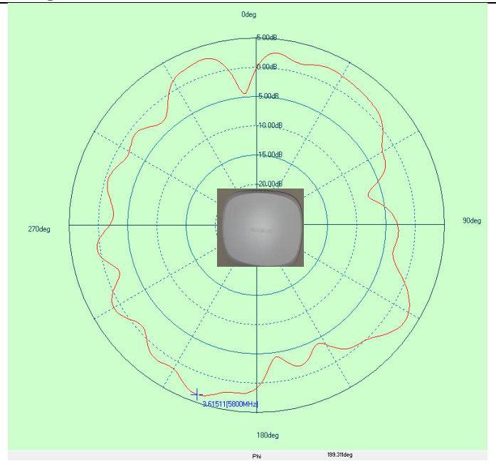
Antenna 1, Dual band (2.4 GHz and 5 GHz) vertical Max gain 3.6 dBi at 5.8 GHz band UNII-3 band
