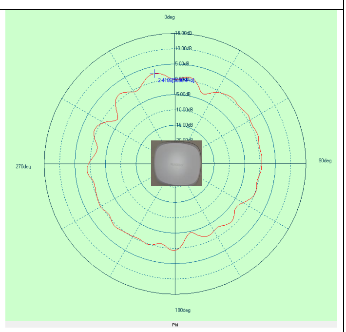
Antennas 3, Dual band (2.4 GHz and 5 GHz) horizontal Max gain 2.4 dBi in 5.8 GHz UNII-3 band
