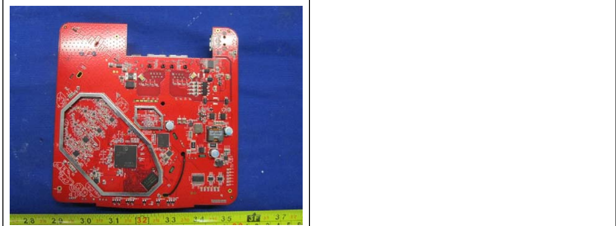
Main Board Bottom View without shielding
