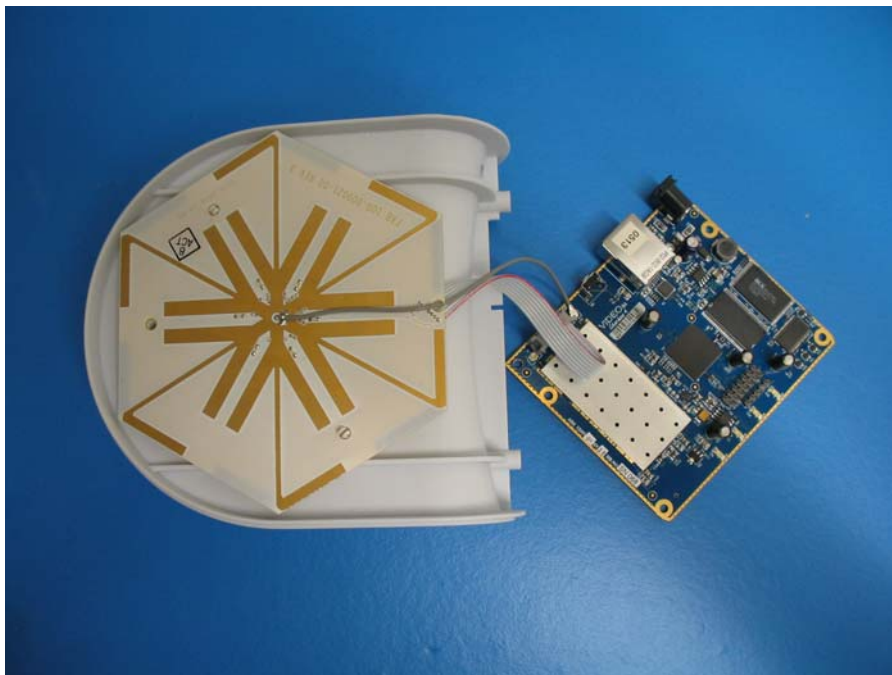
EUT – Top and Bottom View
