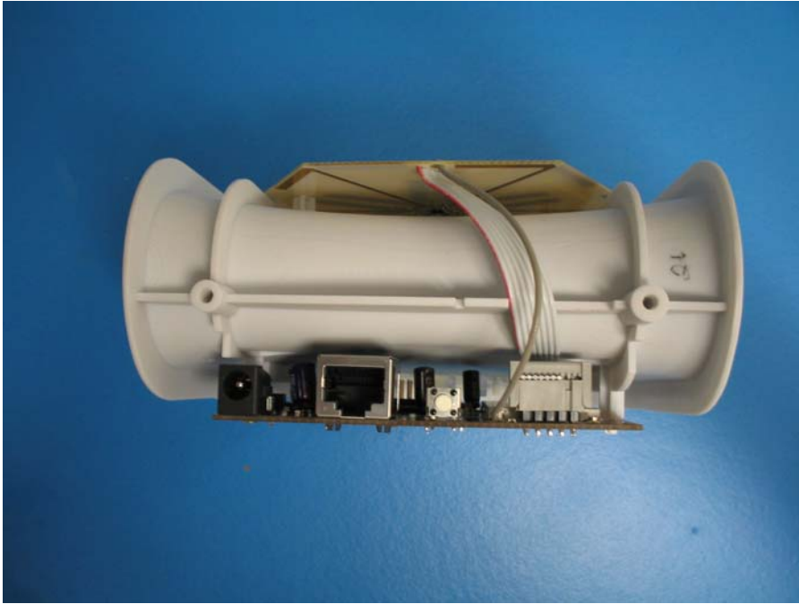
EUT – Internal Rear View
