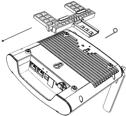
FIGURE 7 Removing the external bracket from the AP
