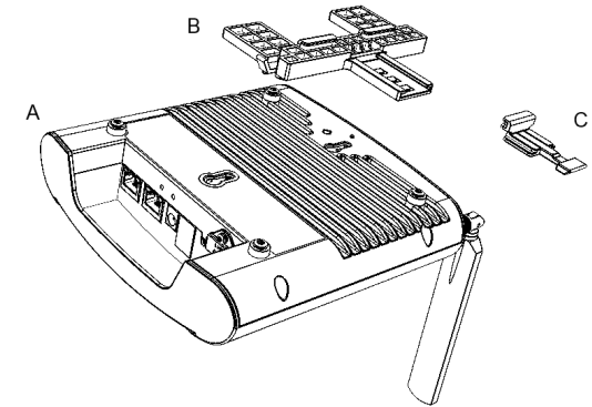
FIGURE 4 Attaching the external bracket to the AP
