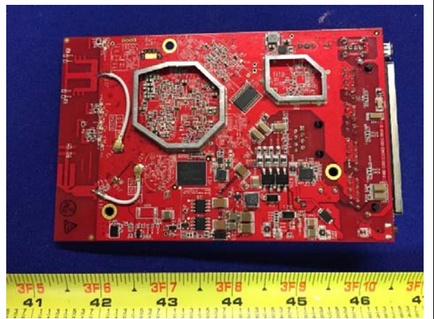
EUT without Shielding Top View
