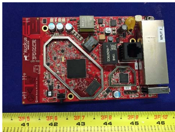
EUT without Shielding Bottom View
