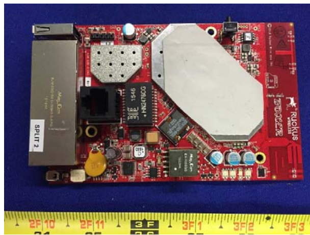
EUT with Shielding Bottom View
