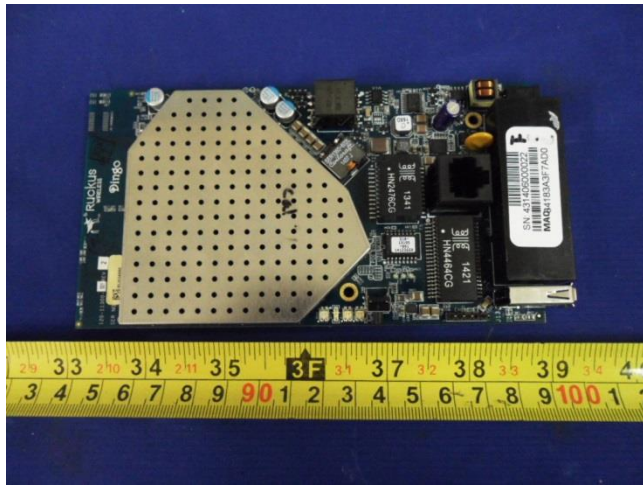
Main Board with Shielding Top View
