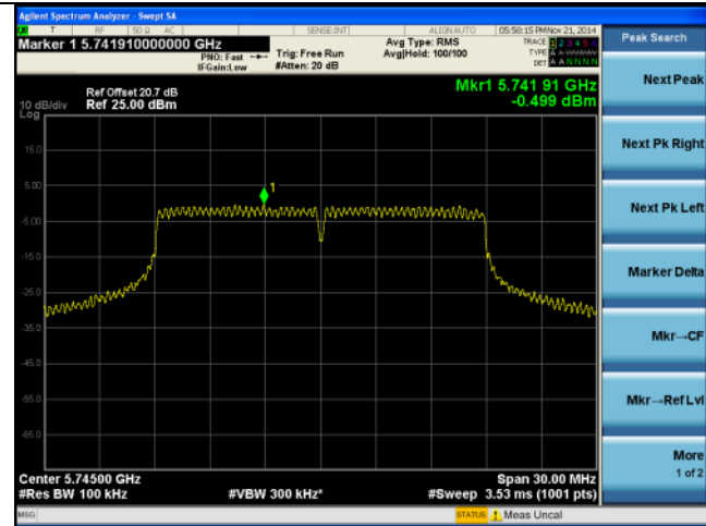
PSD-5.8G-802.11n-20M Low-chain1
