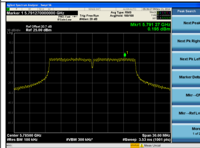
PSD-5.8G-802.11a Mid-chain0
