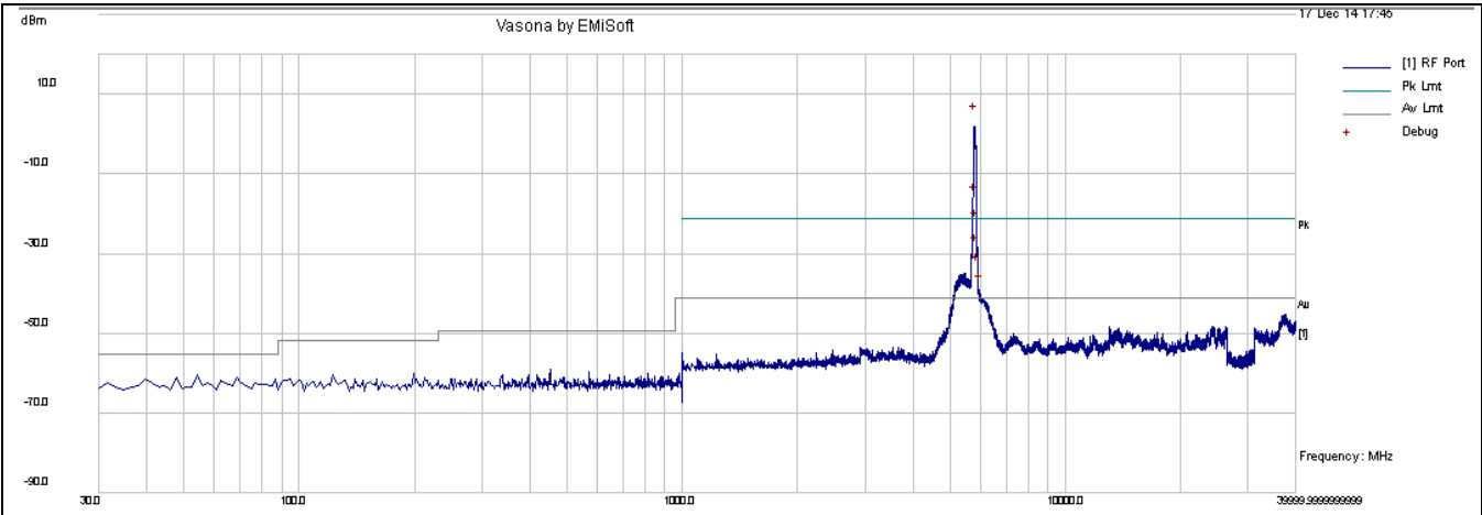
CSE-802.11n-40M 5795MHz-chain1
