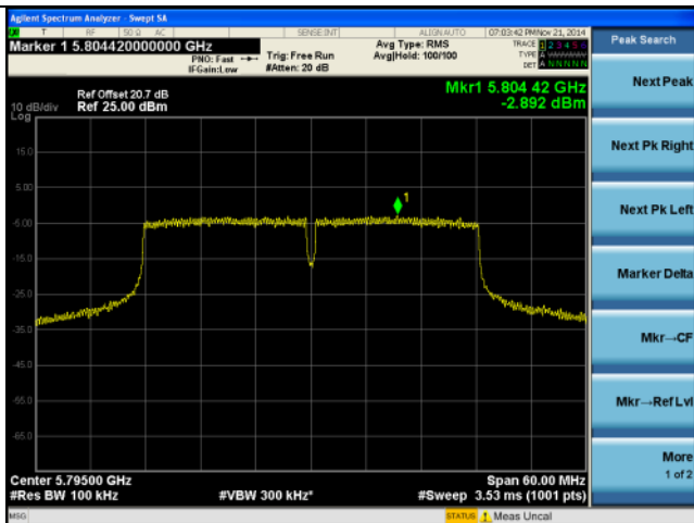
PSD-5.8G-802.11n-40M High-chain0
