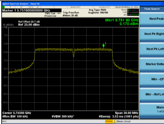
PSD-5.8G-802.11n-20M Low-chain0
