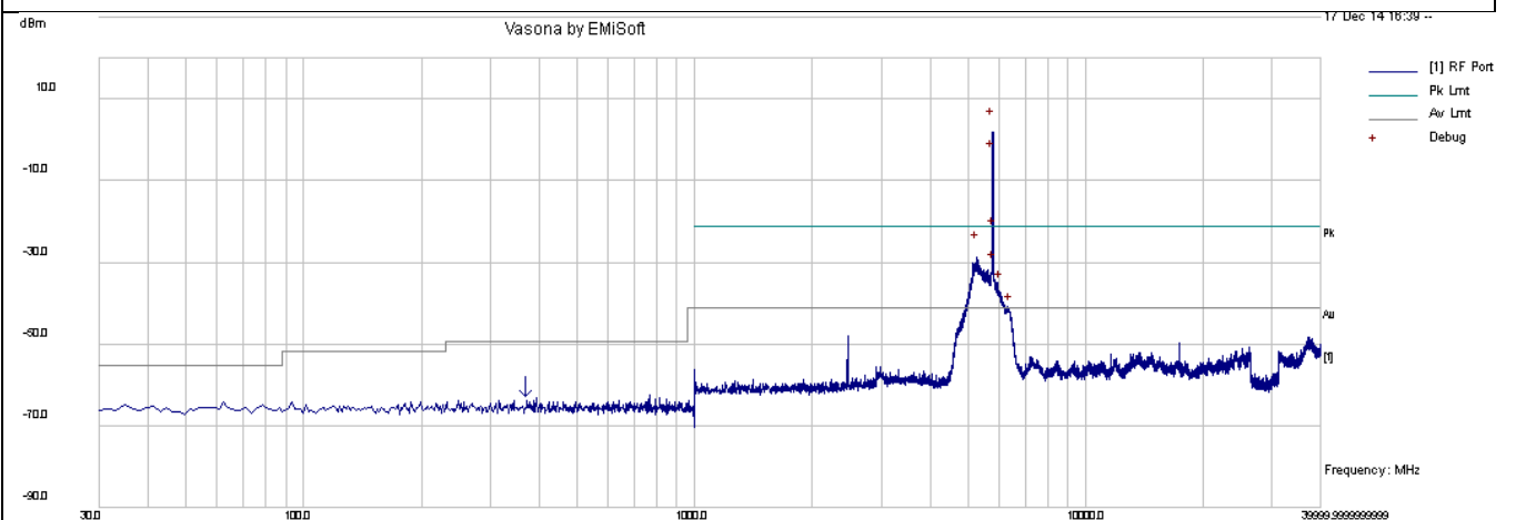
CSE-802.11a 5785MHz-chain0
