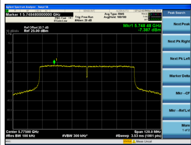
PSD-5.8G-802.11ac-80M Mid-chain1
