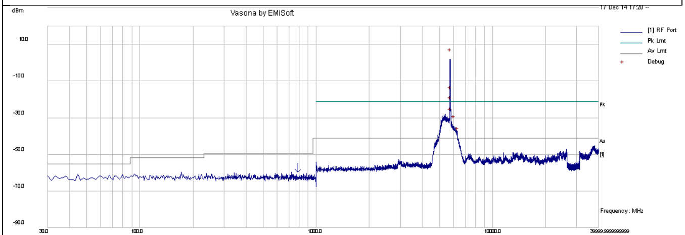
CSE-802.11n-20M 5745MHz-chain1
