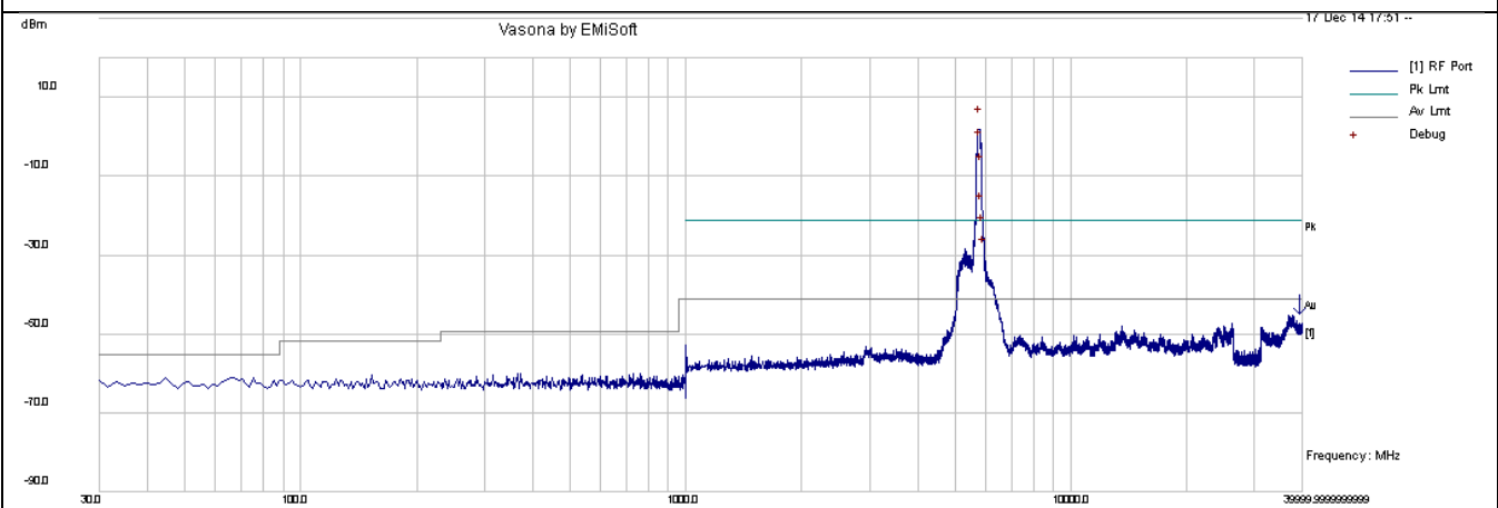
CSE-802.11ac-80M 5775-chain1
