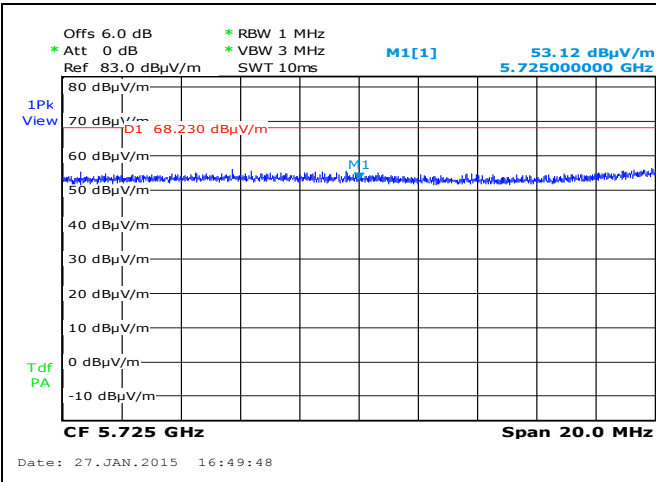
Radiated Band Edge-802.11n 5755M- Edge Freq 5725MHz
