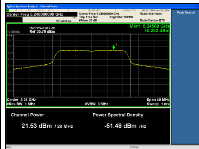
PSD-802.11n-20M-5240M-chain0
