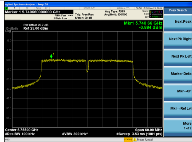
PSD-5.8G-802.11n-40M Low-chain1
