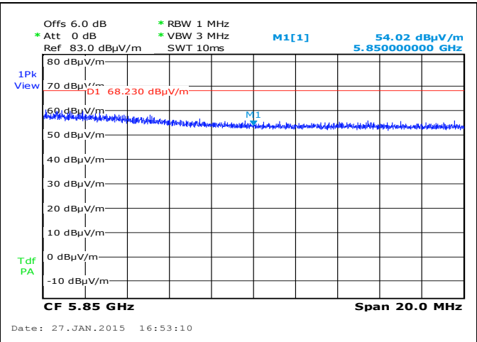
Radiated Band Edge-802.11n 5795M- Edge Freq 5850MHz
