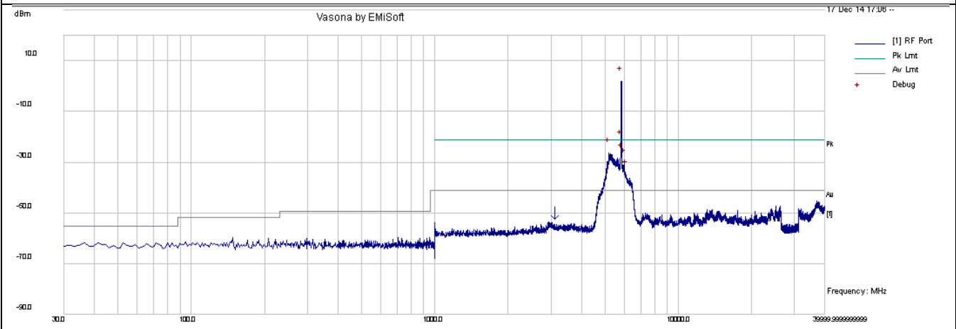
CSE-802.11n-20M 5825MHz-chain0
