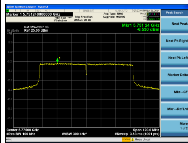
PSD-5.8G-802.11ac-80M Mid-chain0
