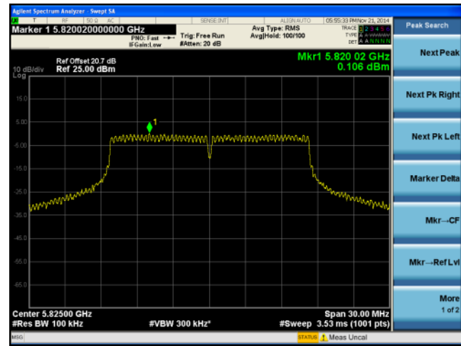
PSD-5.8G-802.11a High-chain1
