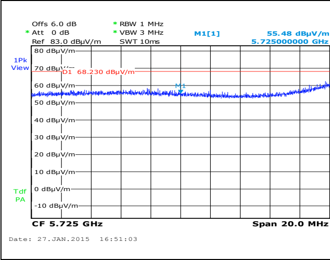
Restricted Band-802.11ac 5750M- Edge Freq 5725MHz
