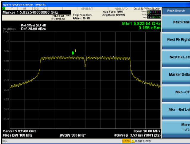
PSD-5.8G-802.11n-20M High-chain0
