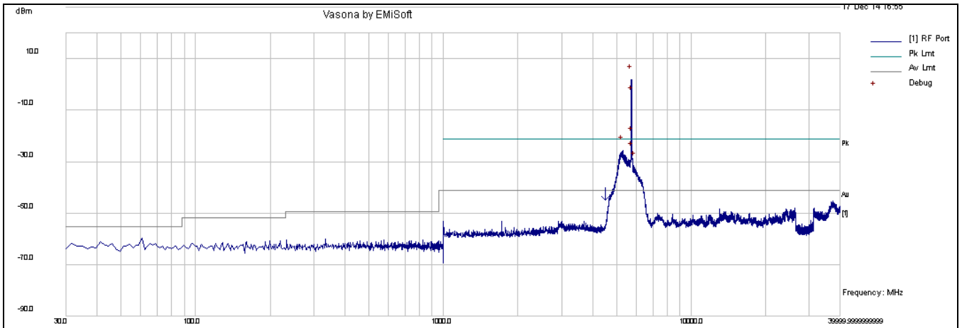
CSE-802.11n-20M 5745MHz-chain0
