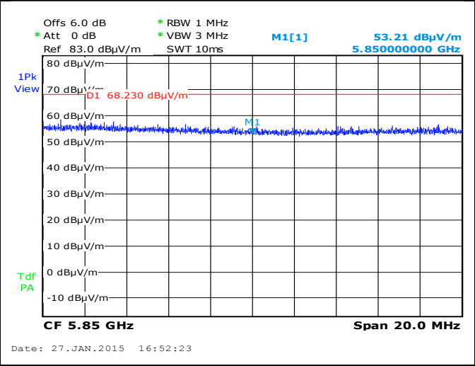
Radiated Band Edge-802.11ac 5775M- Edge Freq 5850MHz
