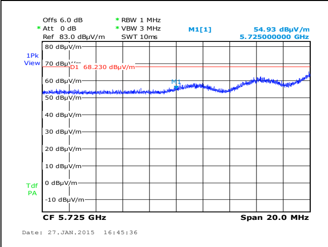
Radiated Band Edge-802.11a 5745M– Edge Freq 5725MHz
