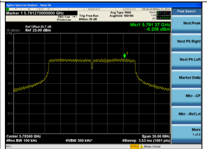
PSD-5.8G-802.11a Mid-chain1
