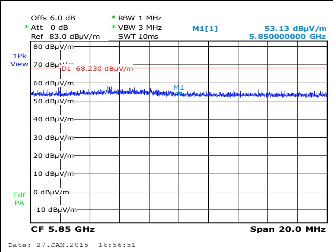
Radiated Band Edge-802.11n 5825M– Edge Freq 5850MHz
