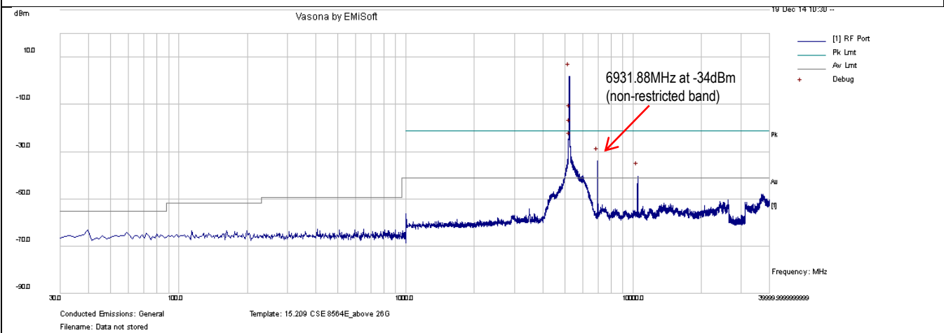
CSE-802.11n-20M 5240MHz-chain1
