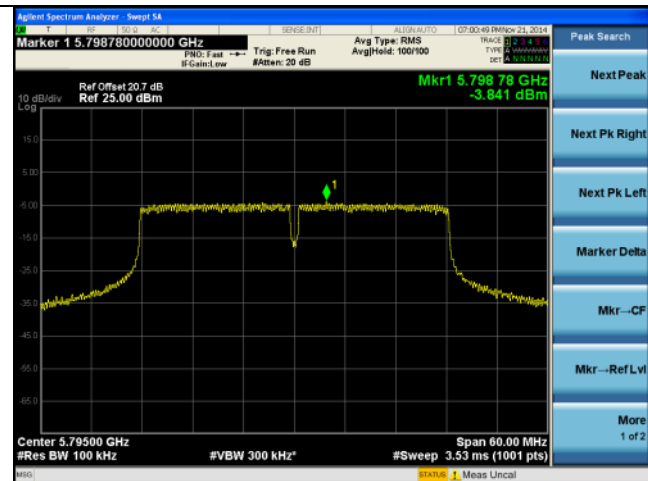
PSD-5.8G-802.11n-40M High-chain1
