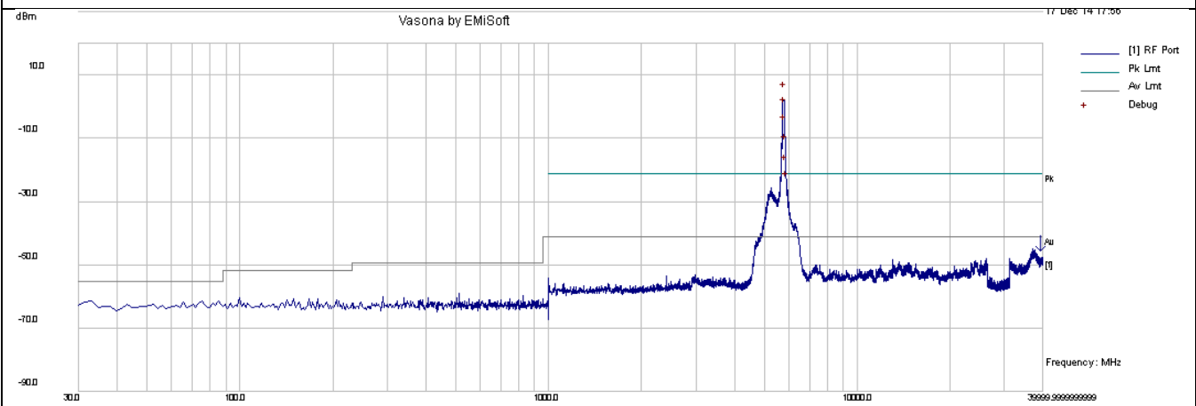
CSE-802.11ac-80M 5775-chain0
