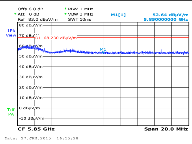
Radiated Band Edge-802.11a 5825M– Edge Freq 5850MHz
