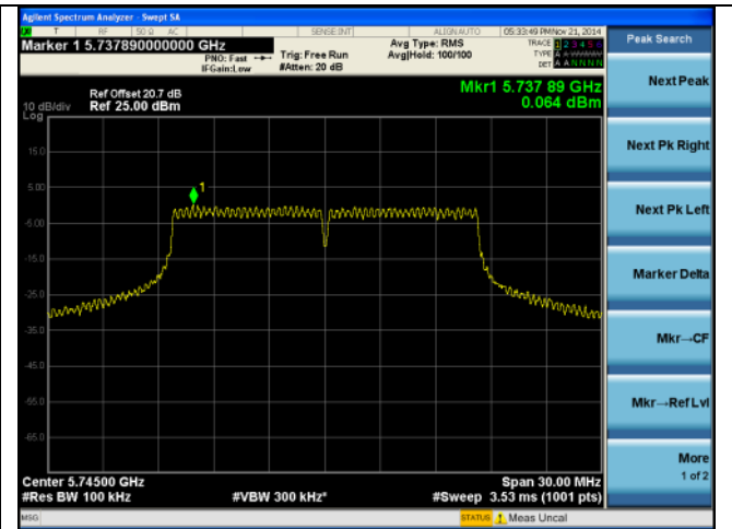
PSD-5.8G-802.11a Low-chain1
