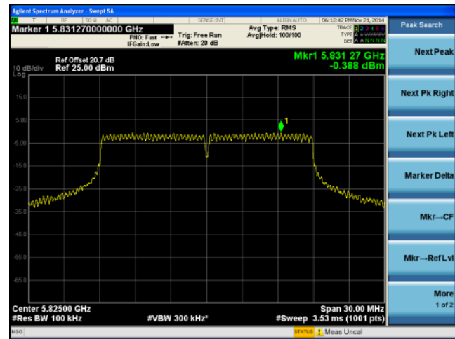
PSD-5.8G-802.11n-20M High-chain1
