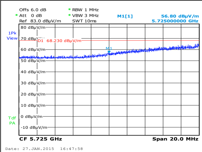
Radiated Band Edge-802.11n 5745M– Edge Freq 5725MHz
