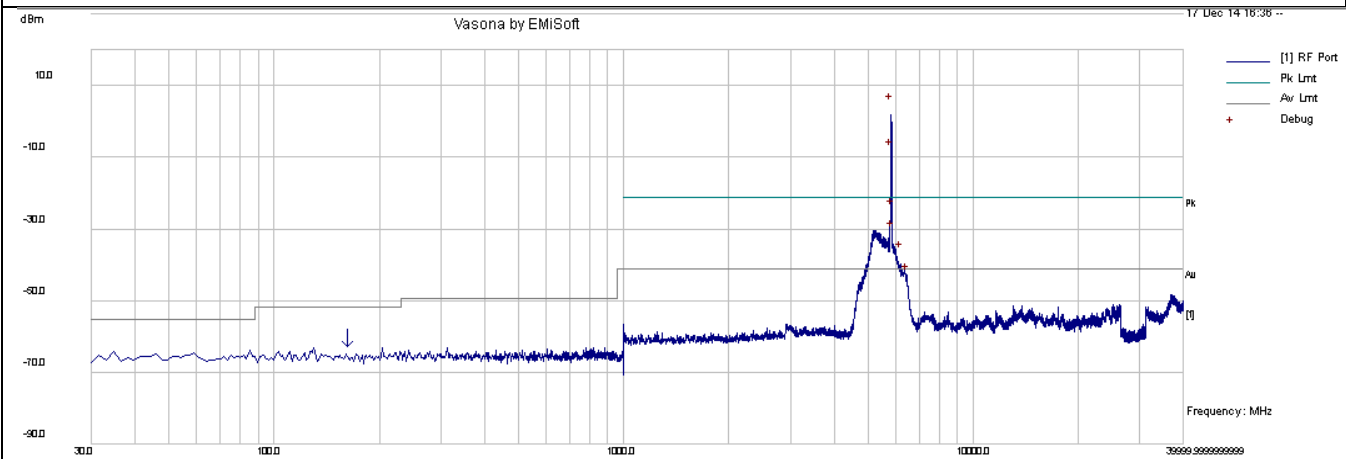
CSE-802.11a 5825MHz-chain0
