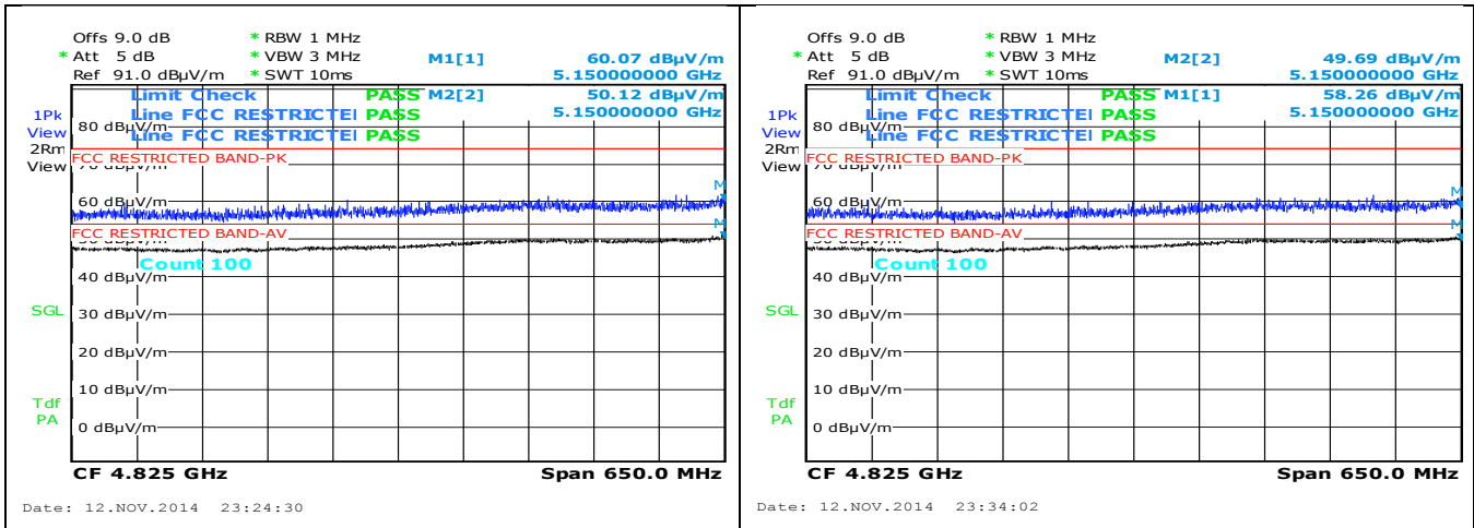
Restricted Band-802.11a 5180M- Edge Freq 5150MHz
