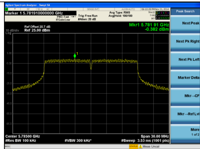
PSD-5.8G-802.11n-20M Mid-chain1
