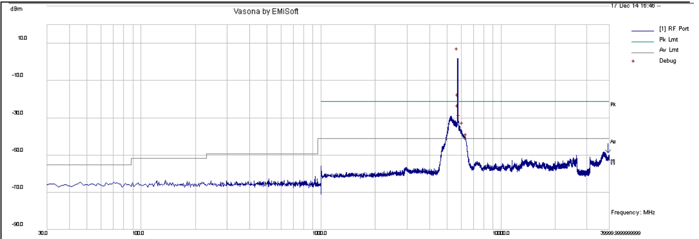
CSE-802.11a 5745MHz-chain0
