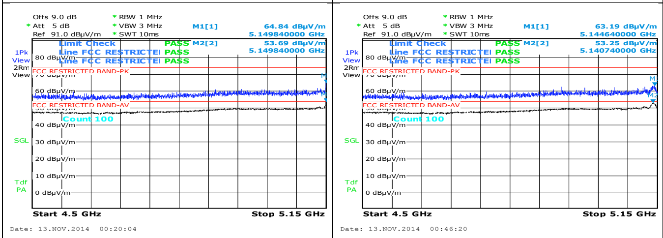
Restricted Band-802.11n-40M 5190M- Edge Freq 5150MHz
