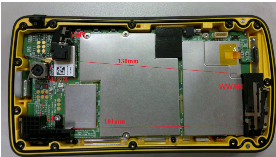
Fig.11 Antenna position of EUT
