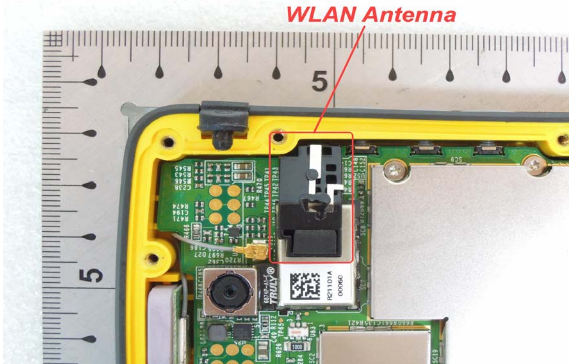
WLAN Antenna
