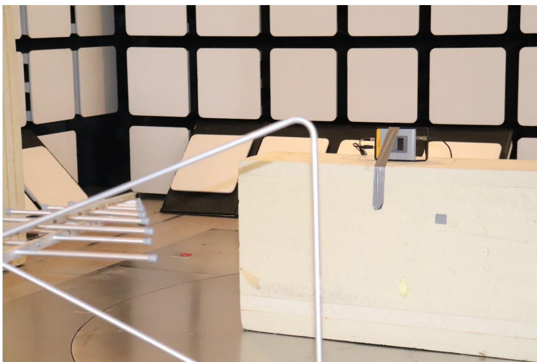
Photograph 5: Radiated emission test setup 30 MHz – 1000 MHz
