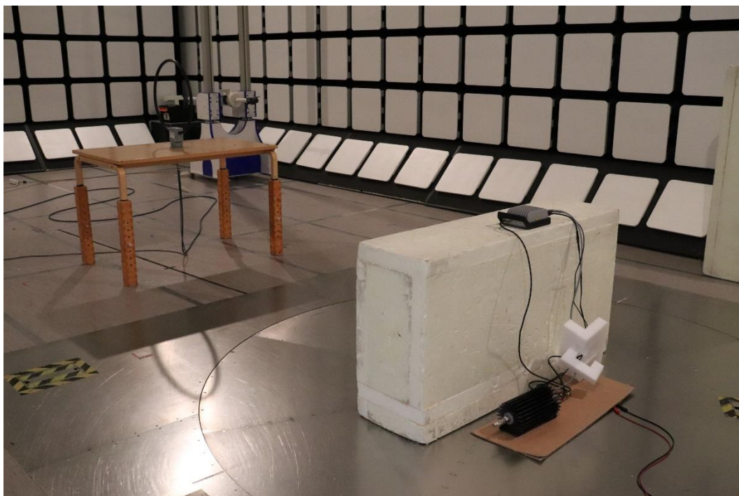
Photograph 4: Radiated emission test setup 9 kHz – 30 MHz
