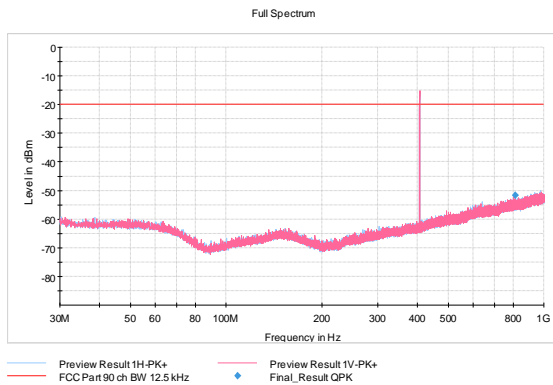
Figure 86: 406.6 MHz, 9600 bps, 12.5 kHz, 1
