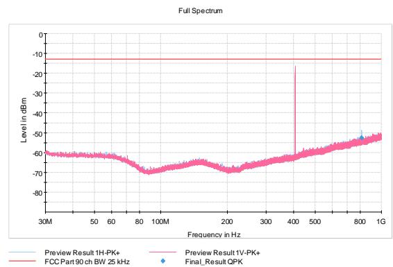
Figure 87: 406.6 MHz, 19200 bps, 25 kHz, 2
