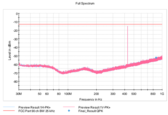
Figure 89: 429.5 MHz, 19200 bps, 25 kHz, 3
