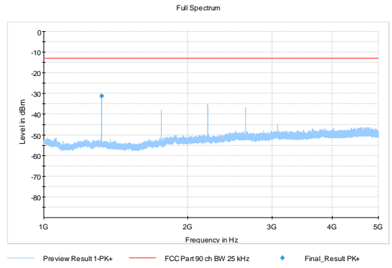
Figure 101: 440.0 MHz, 19200 bps, 25 kHz, 3
