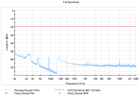
Figure 82: 450.5 MHz, 9600 bps, 12.5 kHz, 2
