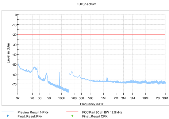
Figure 84: 469.5 MHz, 9600 bps, 12.5 kHz, 3
