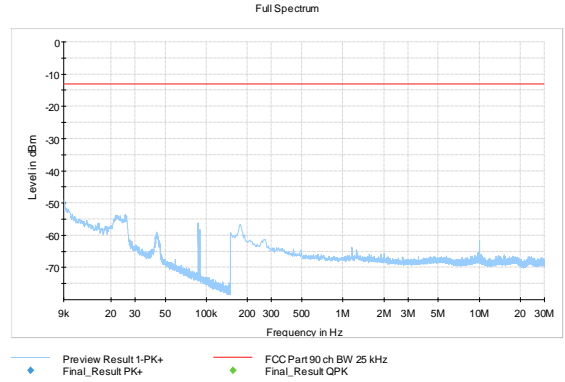
Figure 83: 450.5 MHz, 19200 bps, 25 kHz, 1
