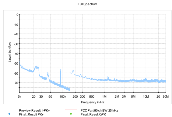
Figure 85: 469.5 MHz, 19200 bps, 25 kHz, 1
