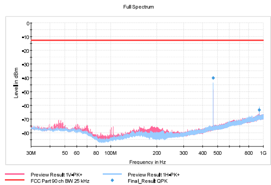
Figure 211: RX 469.5 MHz, 25 kHz, 4800 bps
