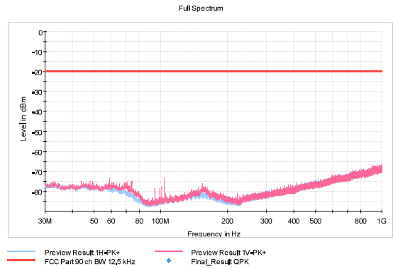
Figure 209: RX 450.5 MHz, 12.5 kHz, 9600 bps
