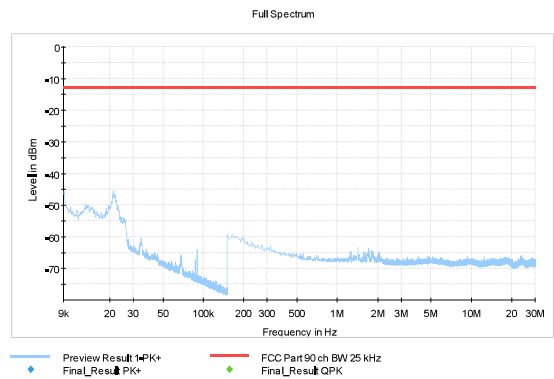
Figure 203: RX 469.5 MHz, 25 kHz, 16000 bps
