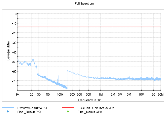
Figure 200: TX 450.5 MHz, 25 kHz, 4800 bps
