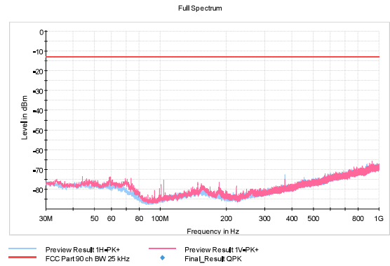
Figure 205: RX 410.0 MHz, 25 kHz, 19200 bps
