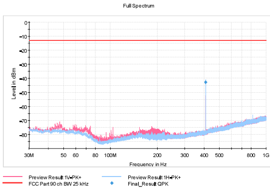
Figure 204: TX 410.0 MHz, 25 kHz, 19200 bps
