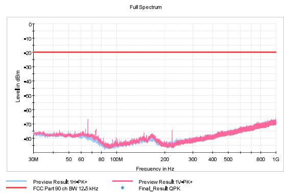
Figure 207: RX 429.5 MHz, 12.5 kHz, 8000 bps
