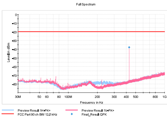
Figure 206: TX 429.5 MHz, 12.5 kHz, 8000 bps
