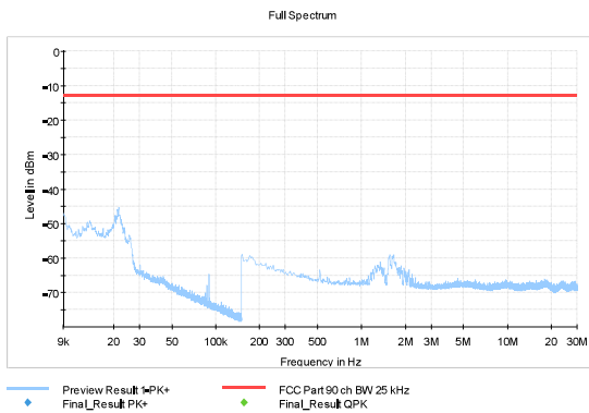
Figure 202: TX 469.5 MHz, 25 kHz, 16000 bps
