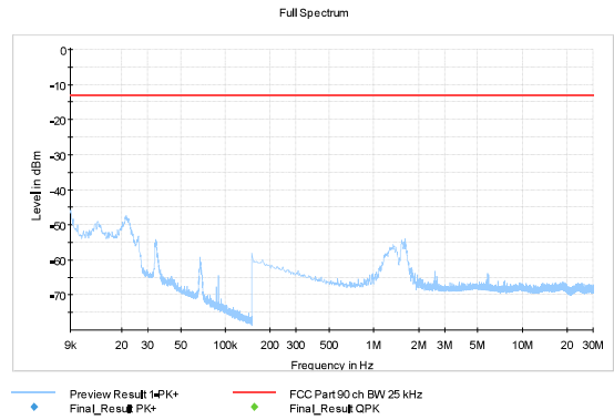
Figure 201: RX 450.5 MHz, 25 kHz, 4800 bps
