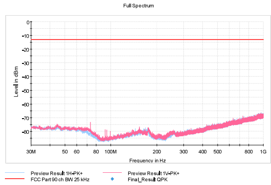
Figure 185: RX 450.5 MHz, 25 kHz, 4FSK
