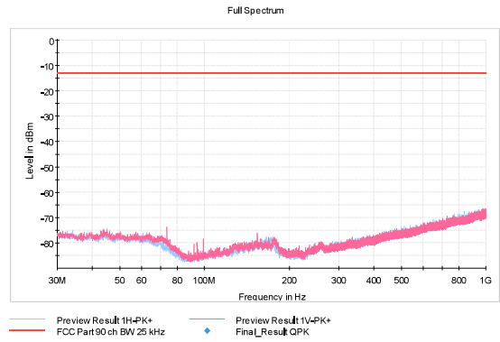
Figure 181: RX 410.0 MHz, 25 kHz, GMSK
