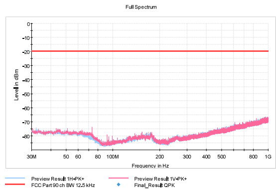
Figure 187: RX 469.5 MHz, 12.5 kHz, 4FSK
