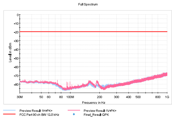
Figure 183: RX 429.5 MHz, 12.5 kHz, GMSK
