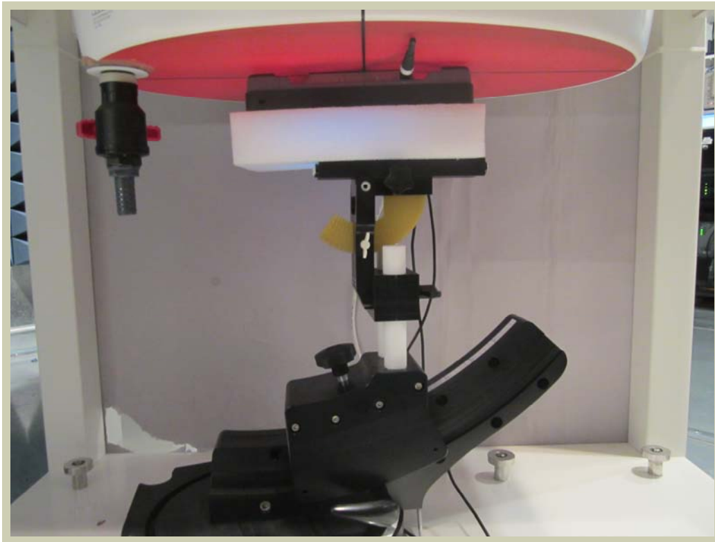
Back of EUT – Antenna Vertical
