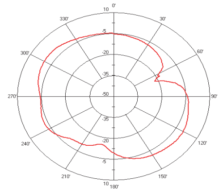
2.45GHz E-Plane Horizontal
