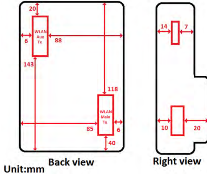
Fig.12 Antenna position of EUT (Back view & Right view)
