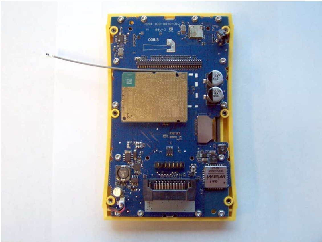
Coax Connected to MC75 Module
