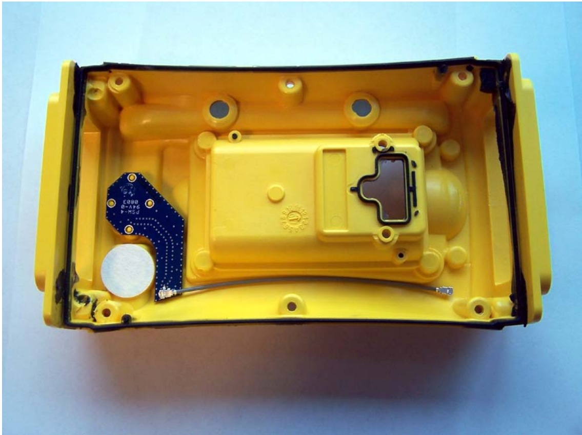
Coax Connected to Antenna Interface PCB
