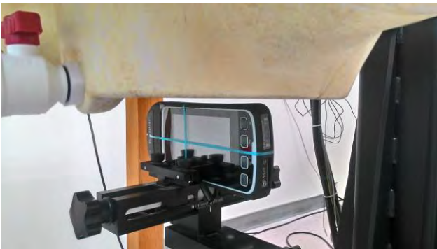
Fig.5 EUT right side to flat phantom
