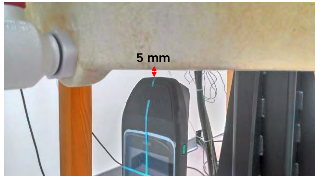
Fig.8 EUT top side to flat phantom
