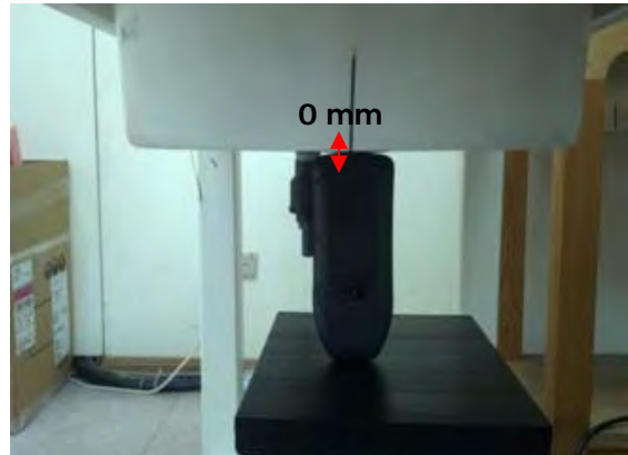
Fig.8 EUT bottom to flat phantom
