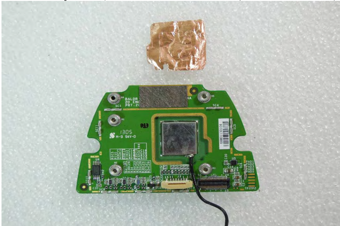
Internal View of EUT-20(Model no.: JUNO/T41/5-BWCSG; JUNO/T41/5-BWCRG)
