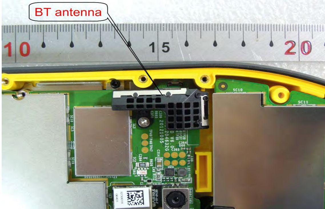
BT Antenna (Model no.: JUNO/T41/5-BWCSG; JUNO/T41/5-BWCRG)
