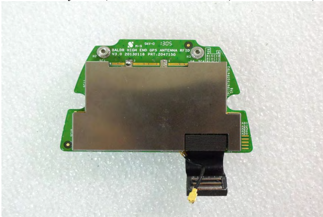
Internal View of EUT-12(Model no.: JUNO/T41/5-BWCSG; JUNO/T41/5-BWCRG)
