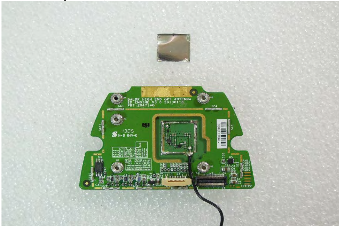
Internal View of EUT-22(Model no.: JUNO/T41/5-BWCSG; JUNO/T41/5-BWCRG)
