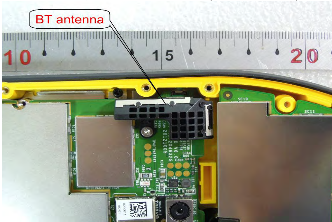
BT Antenna (Model no.: JUNO/T41/5-BWCSG; JUNO/T41/5-BWCRG)
