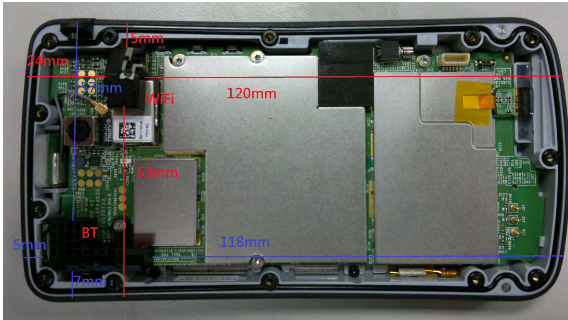
Fig.9 Antenna position of EUT
