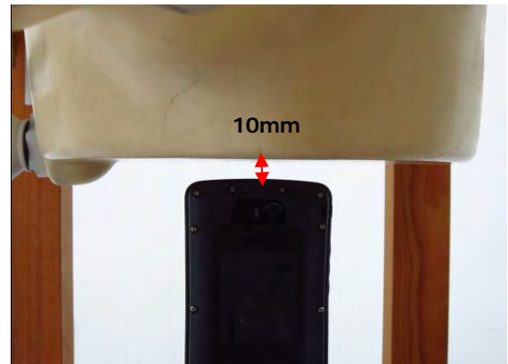
Fig.5 EUT Top to flat phantom
