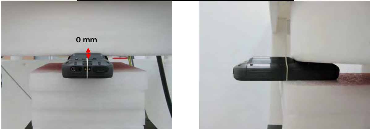
Fig.6 EUT Back side (WLAN Aux) to flat phantom
