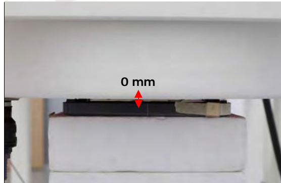
Fig.3 EUT Back side to flat phantom
