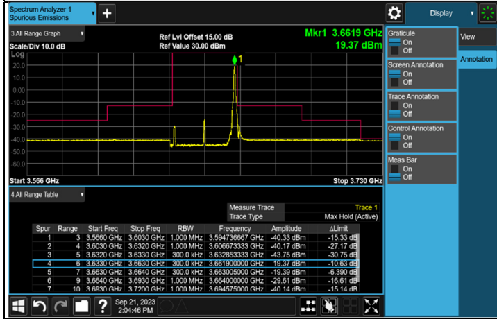
1RB#MAX CH 643200 (3648 MHz)
