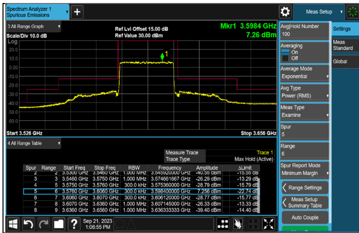
FULL CH 639400 (3591 MHz)
