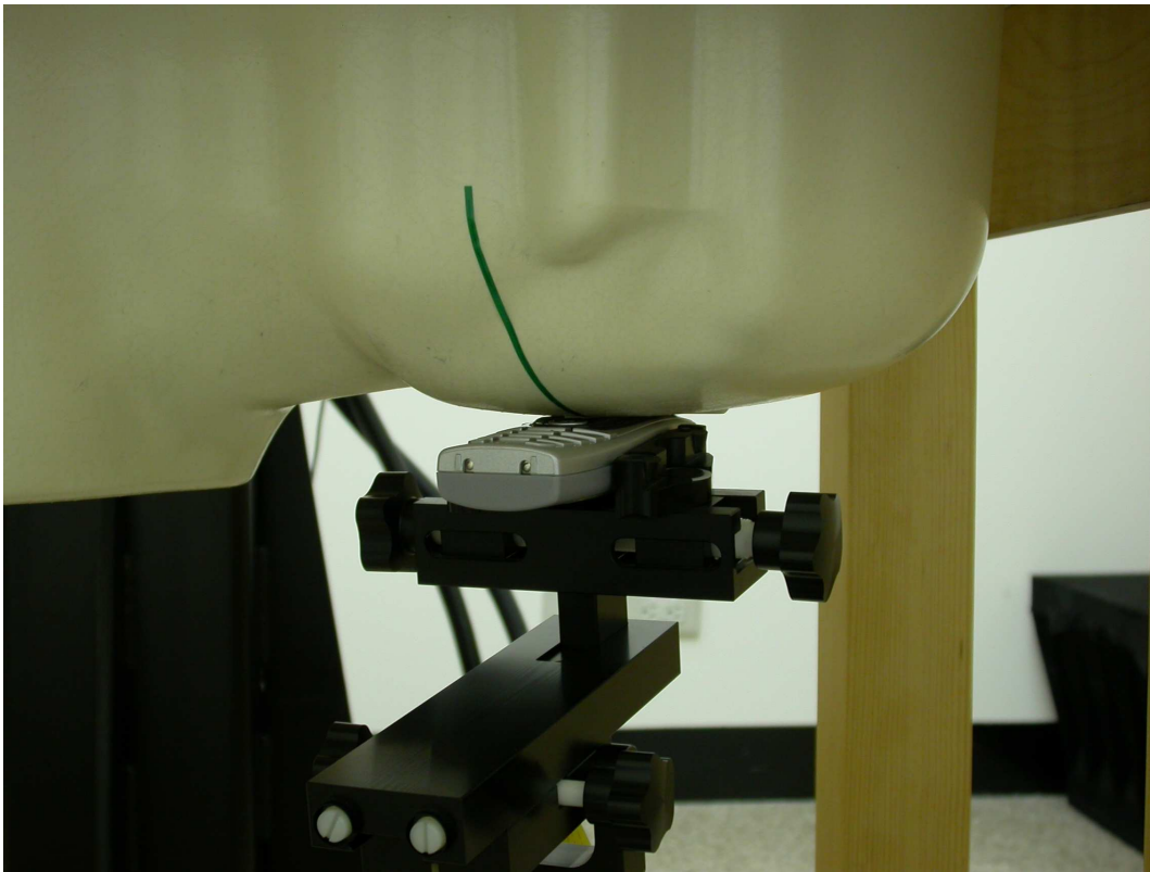
Measurement Position of Left-Cheek (LC) with Handset
