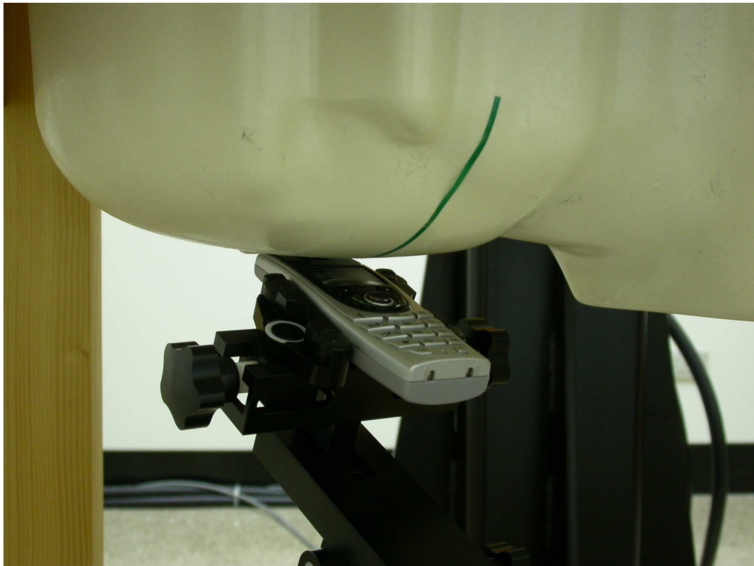
Measurement Position of Right-Tilt (RT) with Handset
