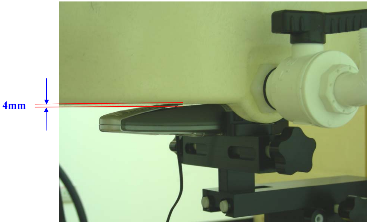
Measurement Position of Rear-UP with Handset
