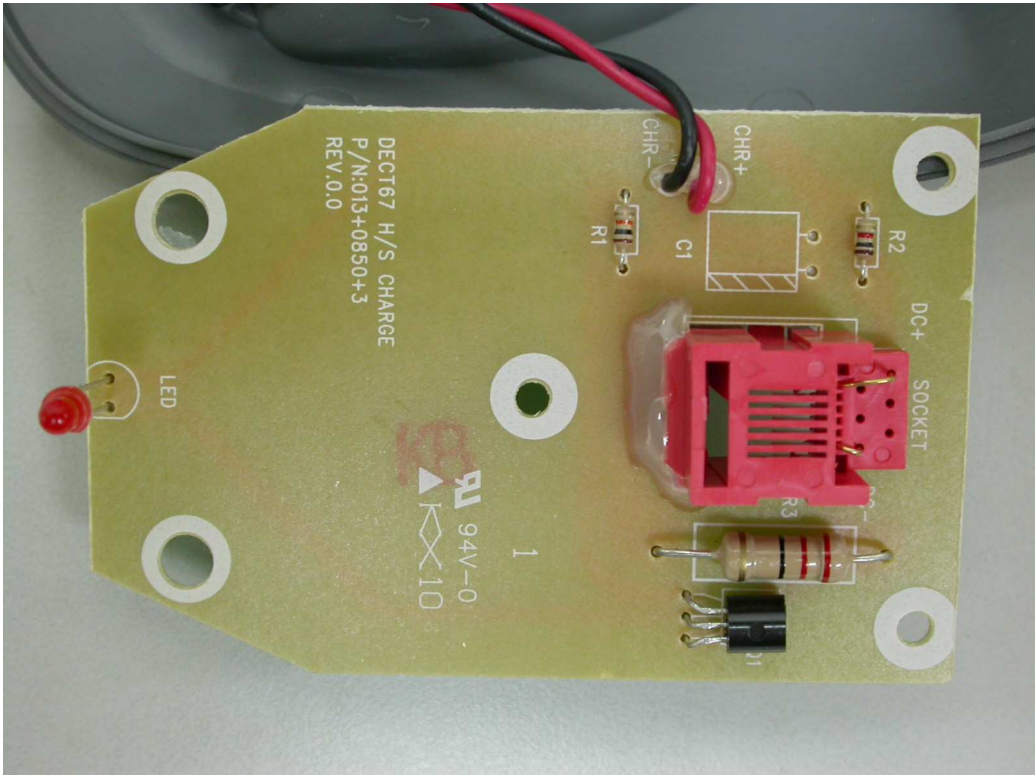
10. Front view of PCB
