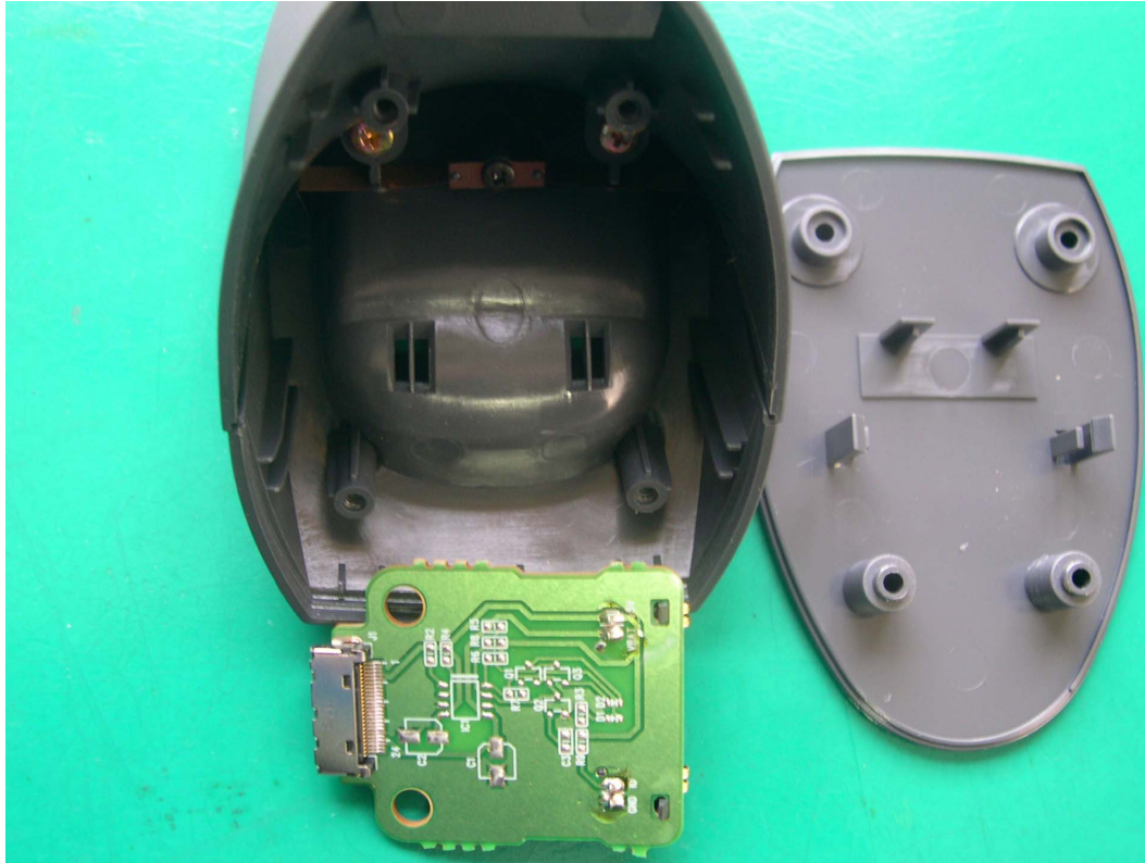
<Photograph 7: Cover removed – Charging cradle >
