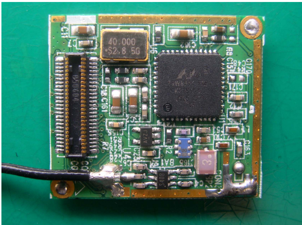
<Photograph 5: Internal Rear View – RF Module >
