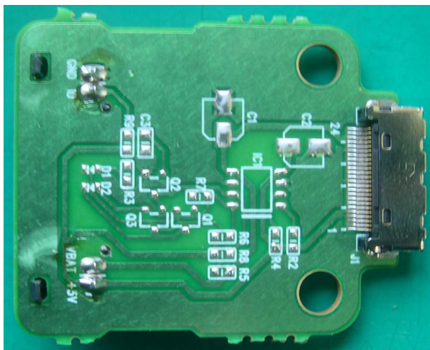
<Photograph 8: Internal PCB Front/Rear View – Charging Cradle >
