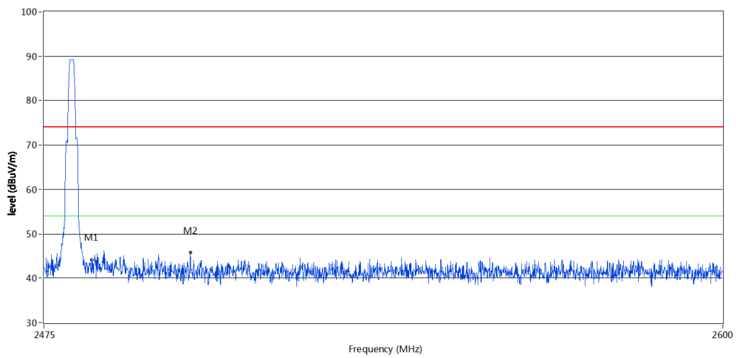
Radiated band-edge_BLE-Band-edge single-H
