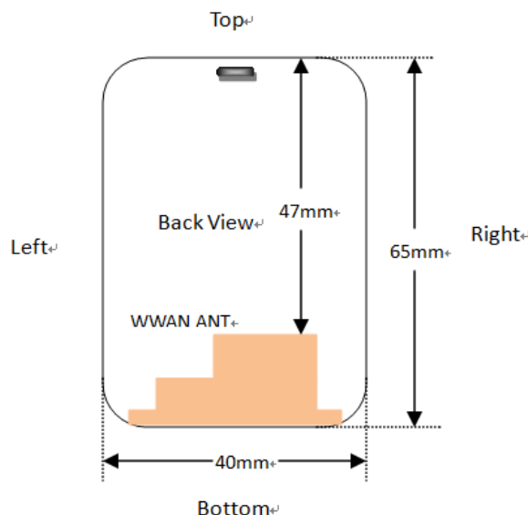
Fig.14.1 EUT Antenna Locations
