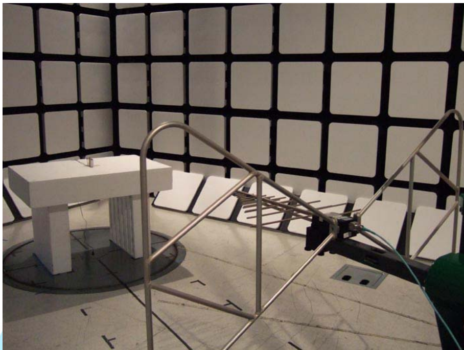
Test Configuration 3: 30 MHz – 960 MHz
