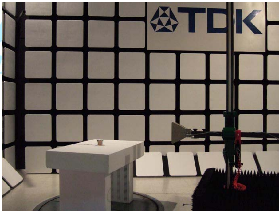
Test Configuration 2: 960 MHz – 40 GHz
