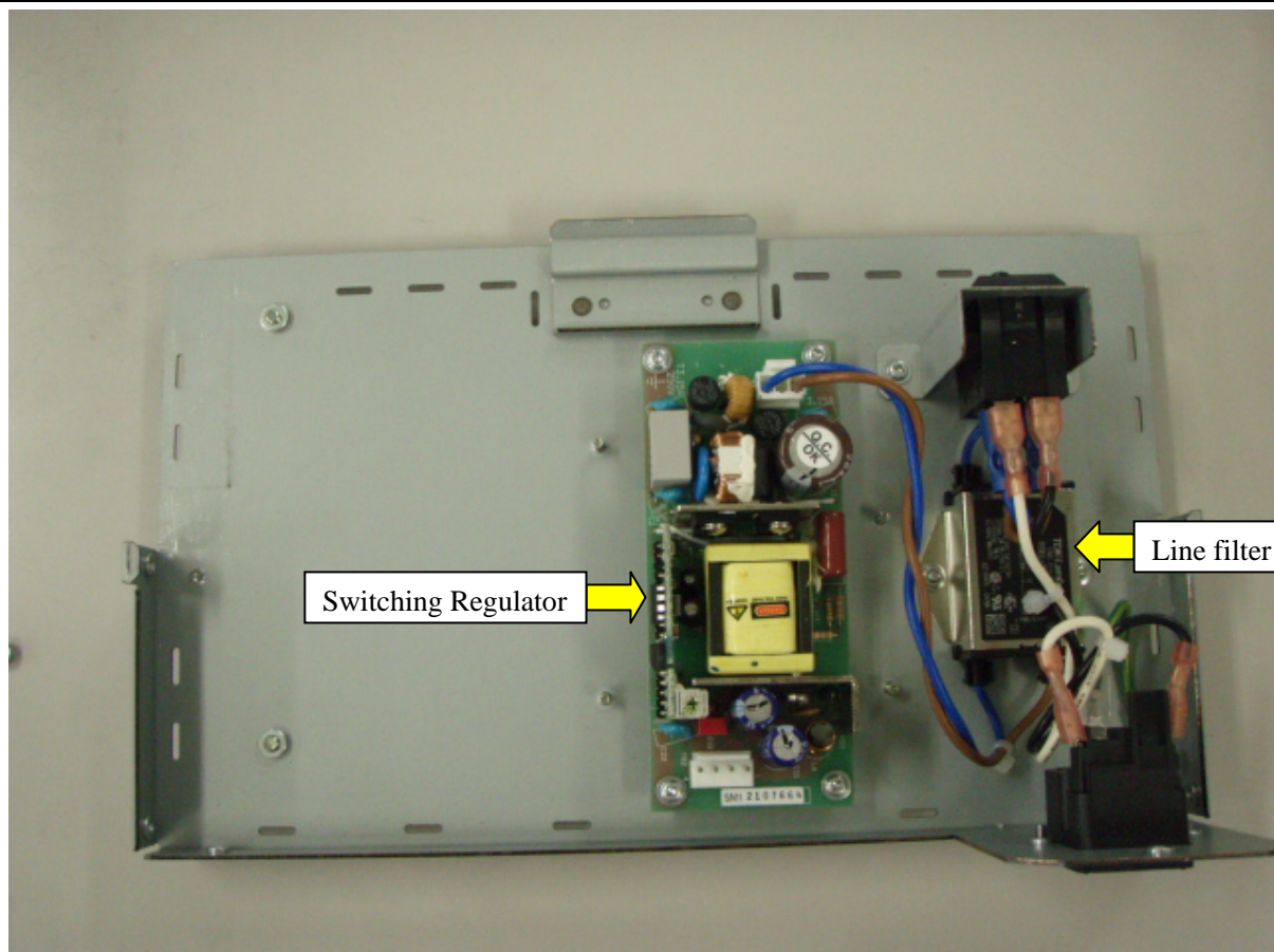
Bottom chassis
