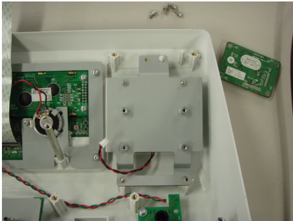
Antenna base (inner side) removing the RFID module
