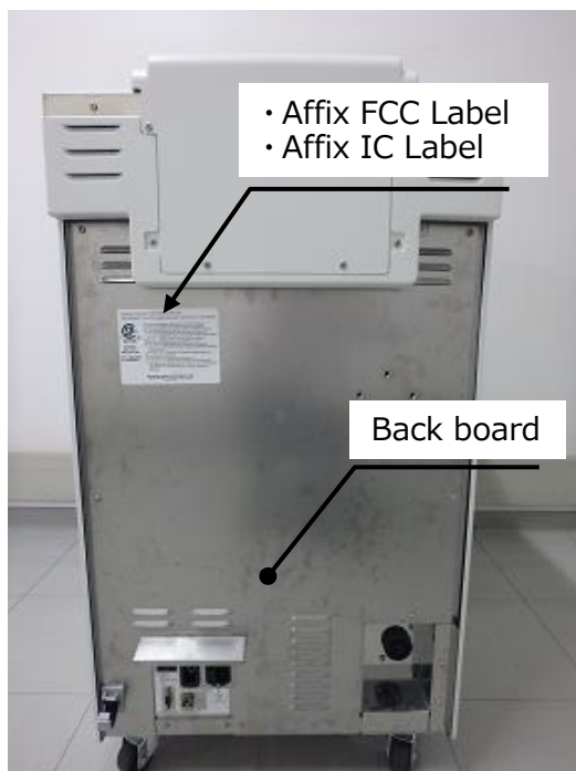
Figure 1: Back of OER-Elite
