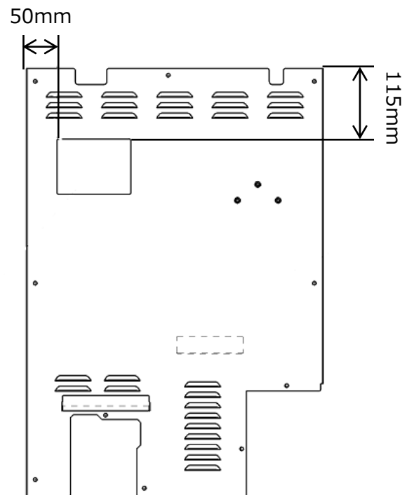
Figure 2: Back board of OER-Elite
